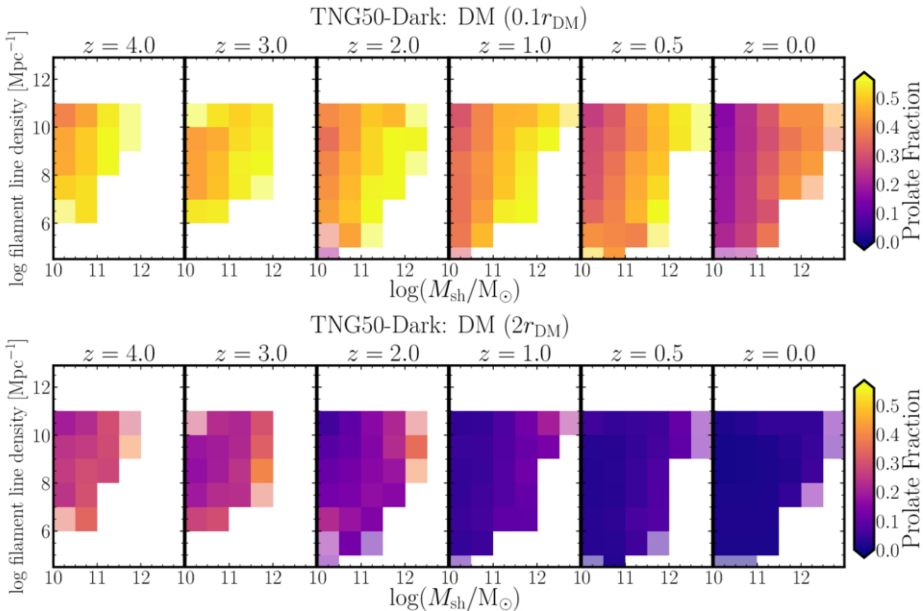
Figure 5. from Farhanul Hasan et al 2026 Astrophys. J. 1004 doi:10.3847/1538-4357/ae60f9 https://dx.doi.org/10.3847/1538-4357/ae60f9 © 2026. The Author(s). Published by the American Astronomical Society.
