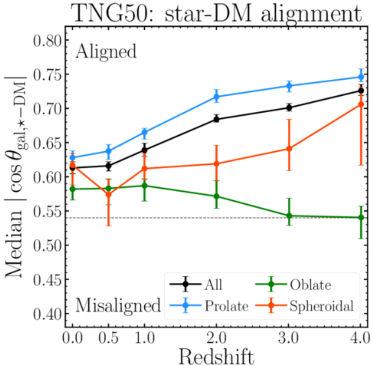
Figure 4. from Farhanul Hasan et al 2026 Astrophys. J. 1004 doi:10.3847/1538-4357/ae60f9 https://dx.doi.org/10.3847/1538-4357/ae60f9 © 2026. The Author(s). Published by the American Astronomical Society.
