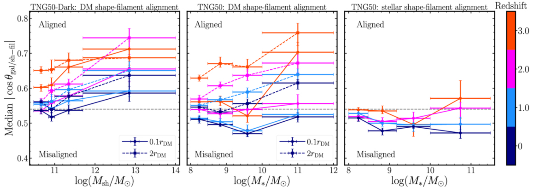
Figure 3. from Farhanul Hasan et al 2026 Astrophys. J. 1004 doi:10.3847/1538-4357/ae60f9 https://dx.doi.org/10.3847/1538-4357/ae60f9 © 2026. The Author(s). Published by the American Astronomical Society.
