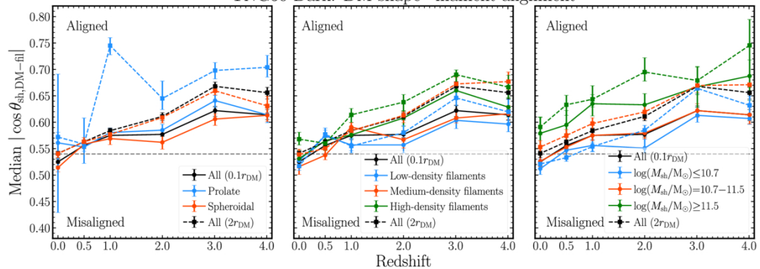
TNG50: DM shape–filament alignment
