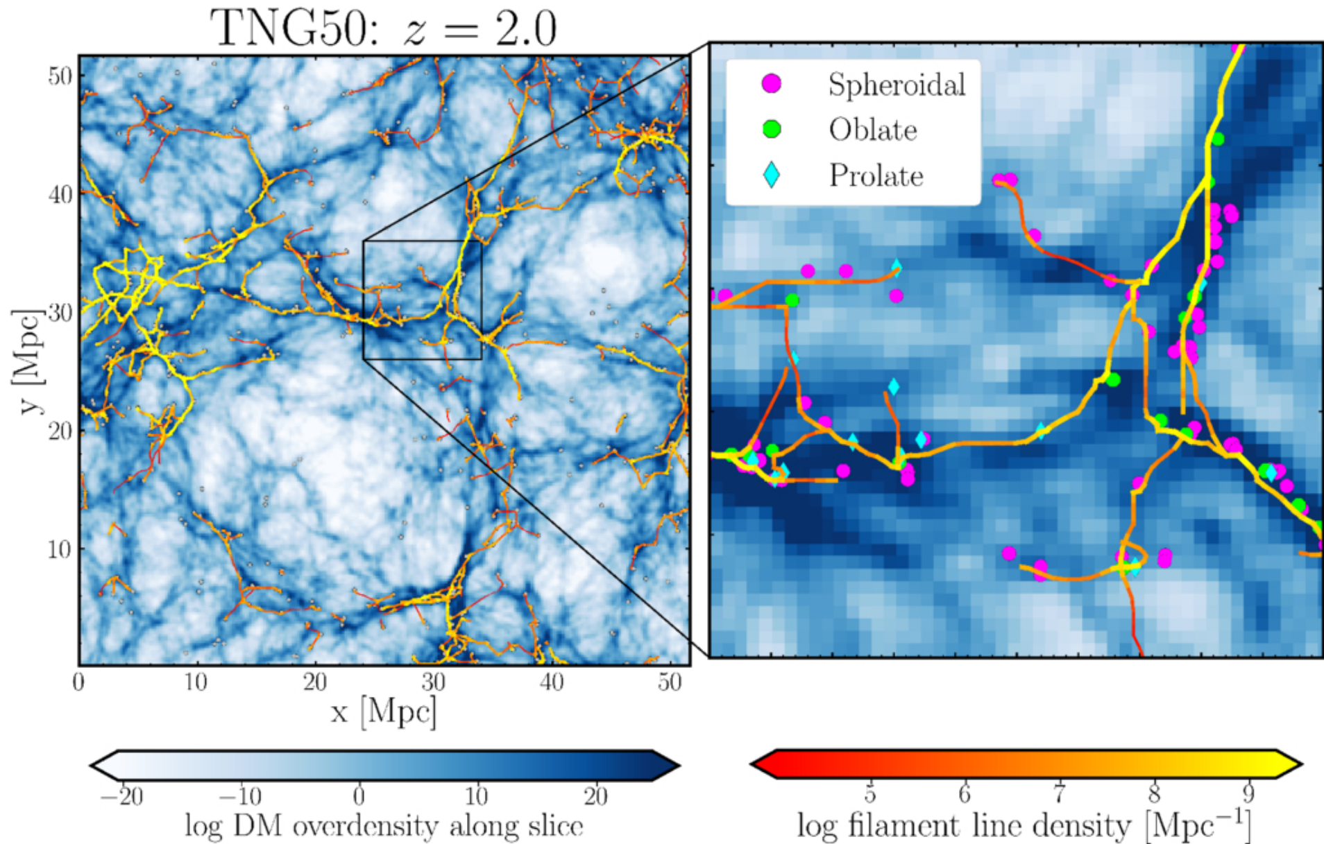
Figure 1. from Farhanul Hasan et al 2026 Astrophys. J. 1004 doi:10.3847/1538-4357/ae60f9 https://dx.doi.org/10.3847/1538-4357/ae60f9 © 2026. The Author(s). Published by the American Astronomical Society.
