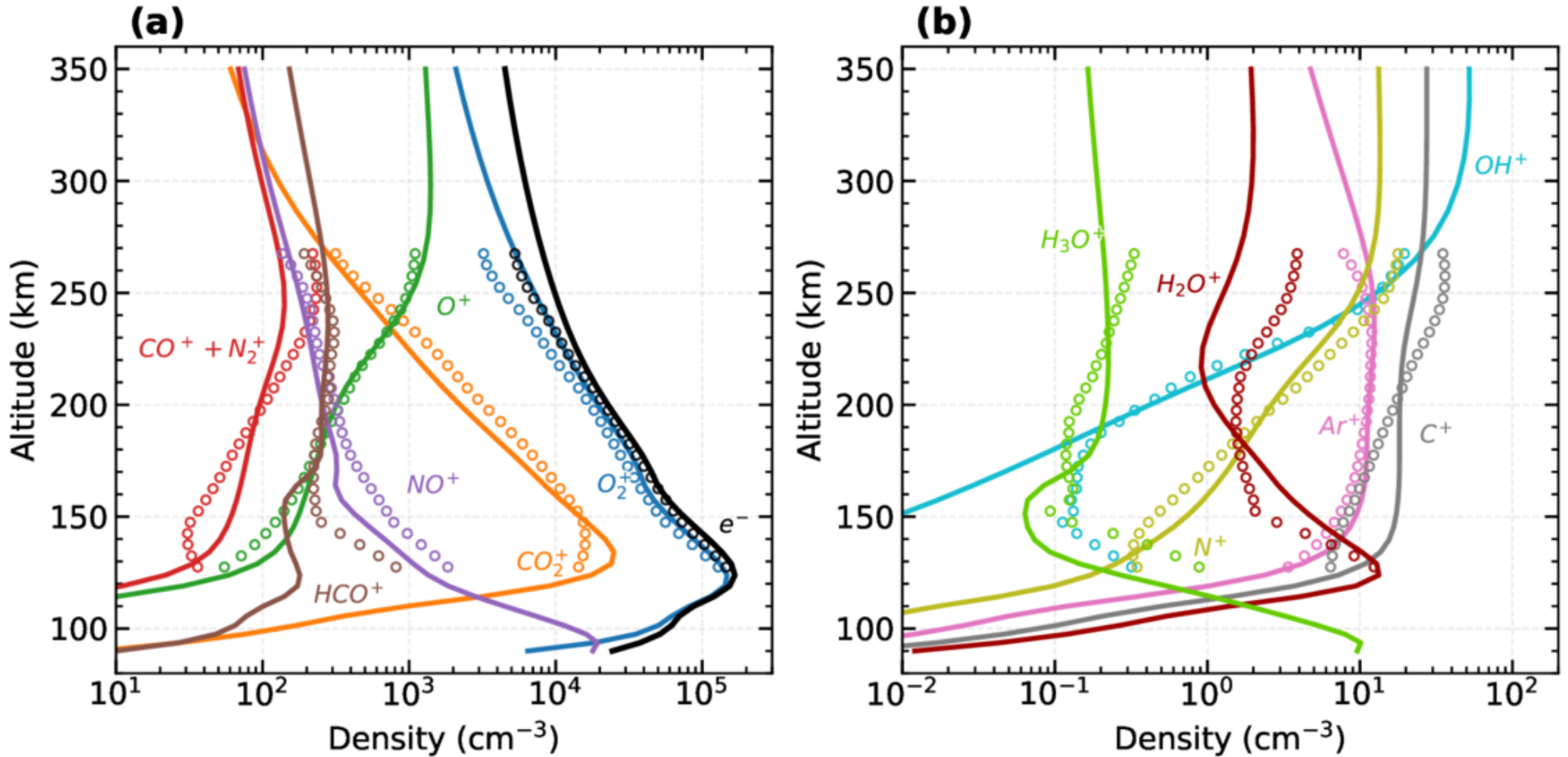
Figure 3. from Yanxing Liu et al 2026 Astrophys. J. 1002 doi:10.3847/1538-4357/ae6070 https://dx.doi.org/10.3847/1538-4357/ae6070 © 2026. The Author(s). Published by the American Astronomical Society.
