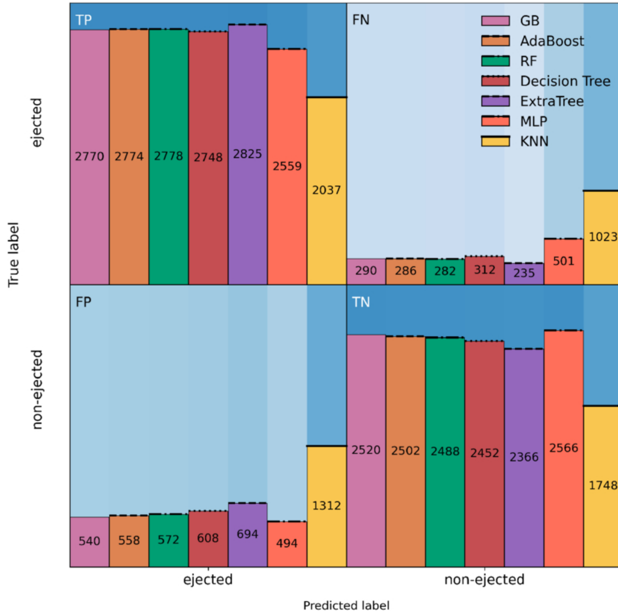
Figure 5. from Chetan Abhijnanam Bora et al 2026 Astrophys. J. 1002 doi:10.3847/1538-4357/ae606f https://dx.doi.org/10.3847/1538-4357/ae606f © 2026. The Author(s). Published by the American Astronomical Society.
