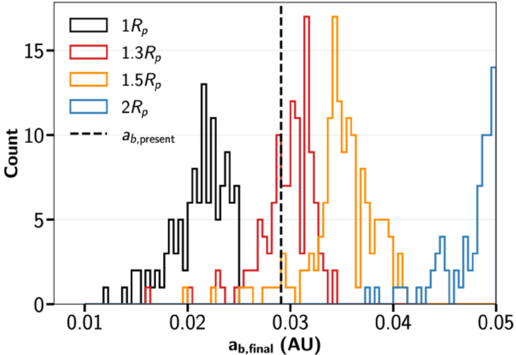
Figure 9. from Haedam Im et al 2026 Astrophys. J. 1003 doi:10.3847/1538-4357/ae606b https://dx.doi.org/10.3847/1538-4357/ae606b © 2026. The Author(s). Published by the American Astronomical Society.
