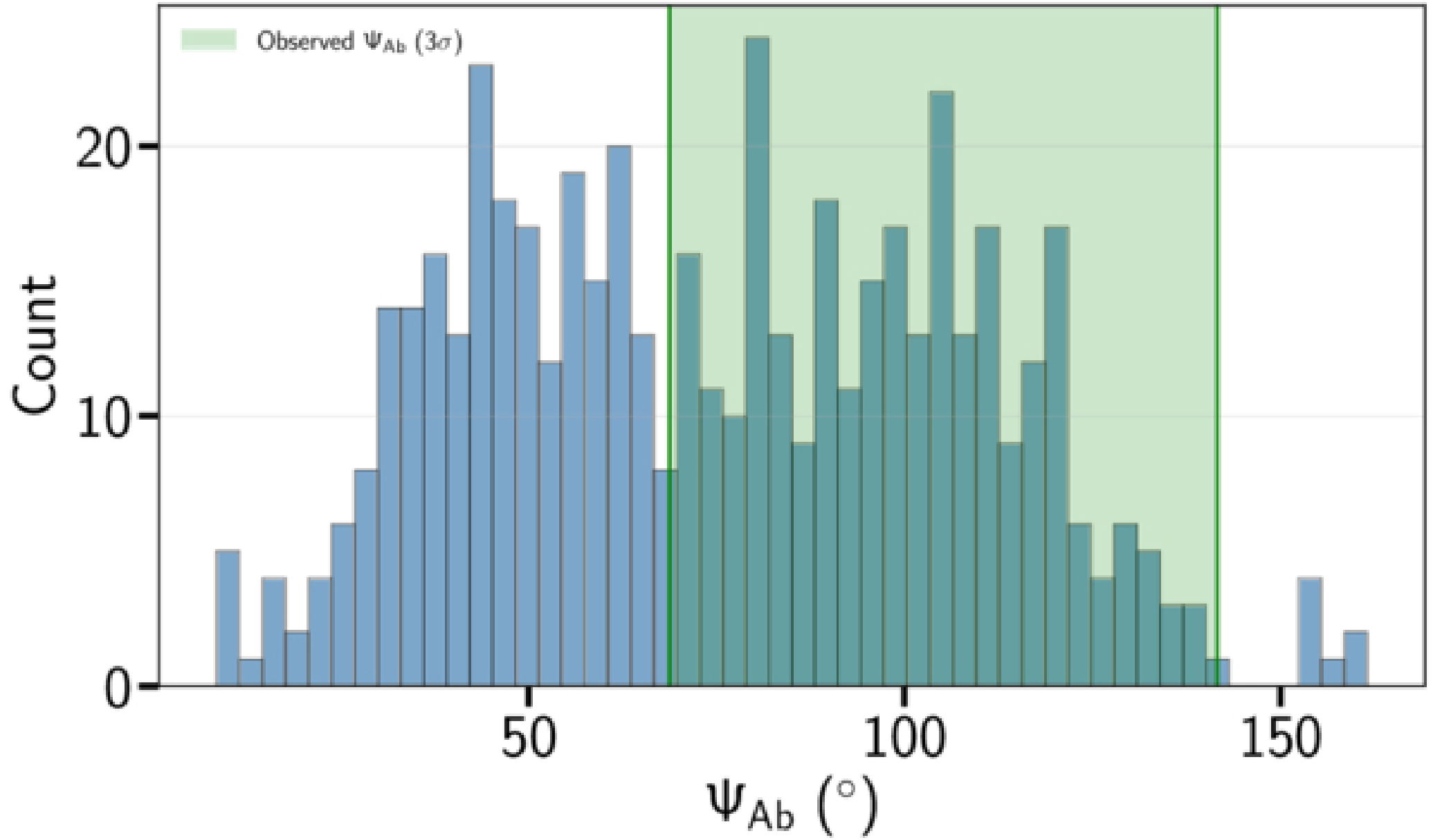
Figure 7. from Haedam Im et al 2026 Astrophys. J. 1003 doi:10.3847/1538-4357/ae606b https://dx.doi.org/10.3847/1538-4357/ae606b © 2026. The Author(s). Published by the American Astronomical Society.
