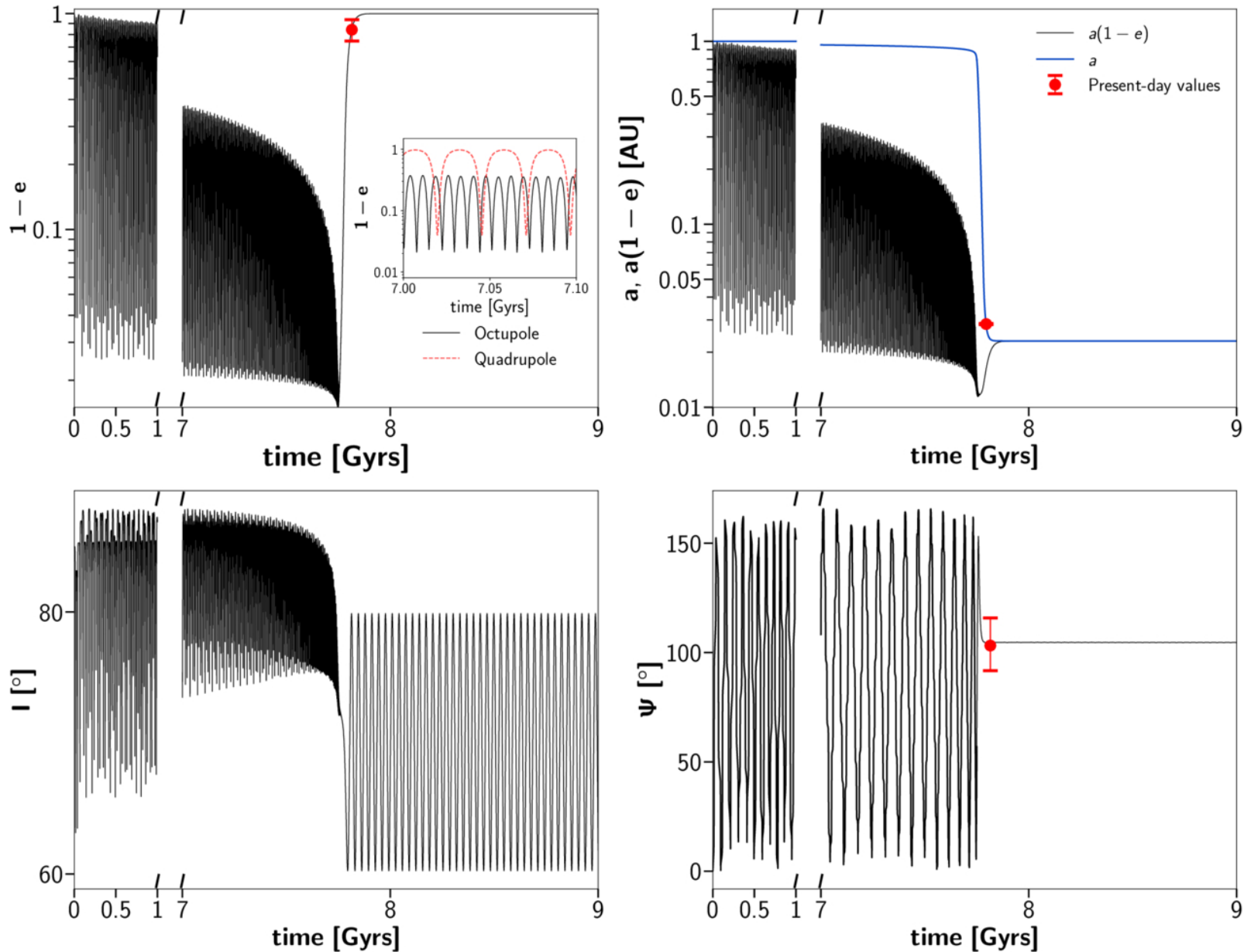
Figure 4. from Haedam Im et al 2026 Astrophys. J. 1003 doi:10.3847/1538-4357/ae606b https://dx.doi.org/10.3847/1538-4357/ae606b © 2026. The Author(s). Published by the American Astronomical Society.
