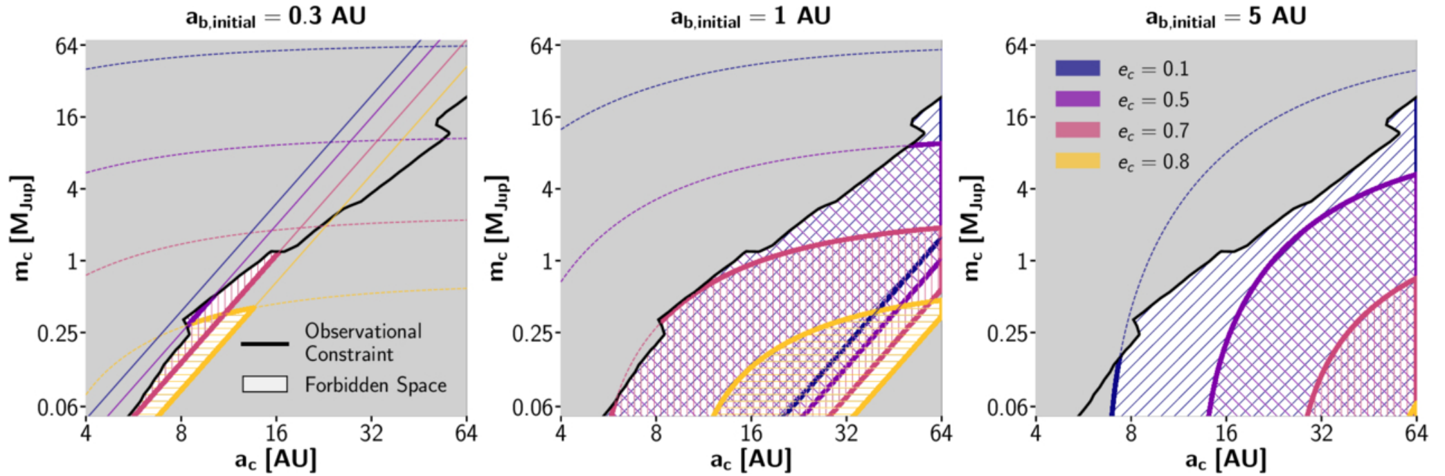
Figure 3. from Haedam Im et al 2026 Astrophys. J. 1003 doi:10.3847/1538-4357/ae606b https://dx.doi.org/10.3847/1538-4357/ae606b © 2026. The Author(s). Published by the American Astronomical Society.
