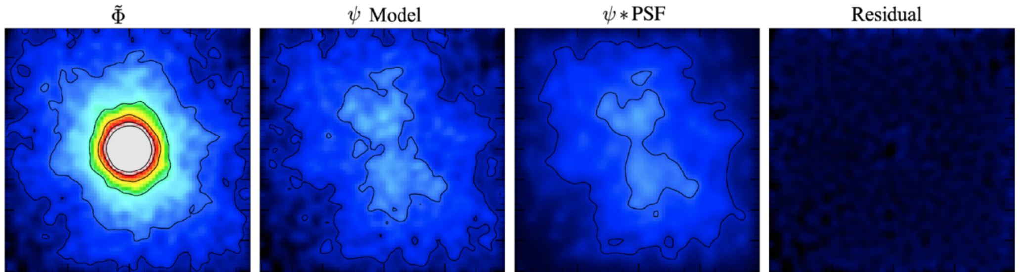
Figure 4. from Kevin Hall and Hai Fu 2026 Astrophys. J. 1002 doi:10.3847/1538-4357/ae6065 https://dx.doi.org/10.3847/1538-4357/ae6065 © 2026. The Author(s). Published by the American Astronomical Society.
