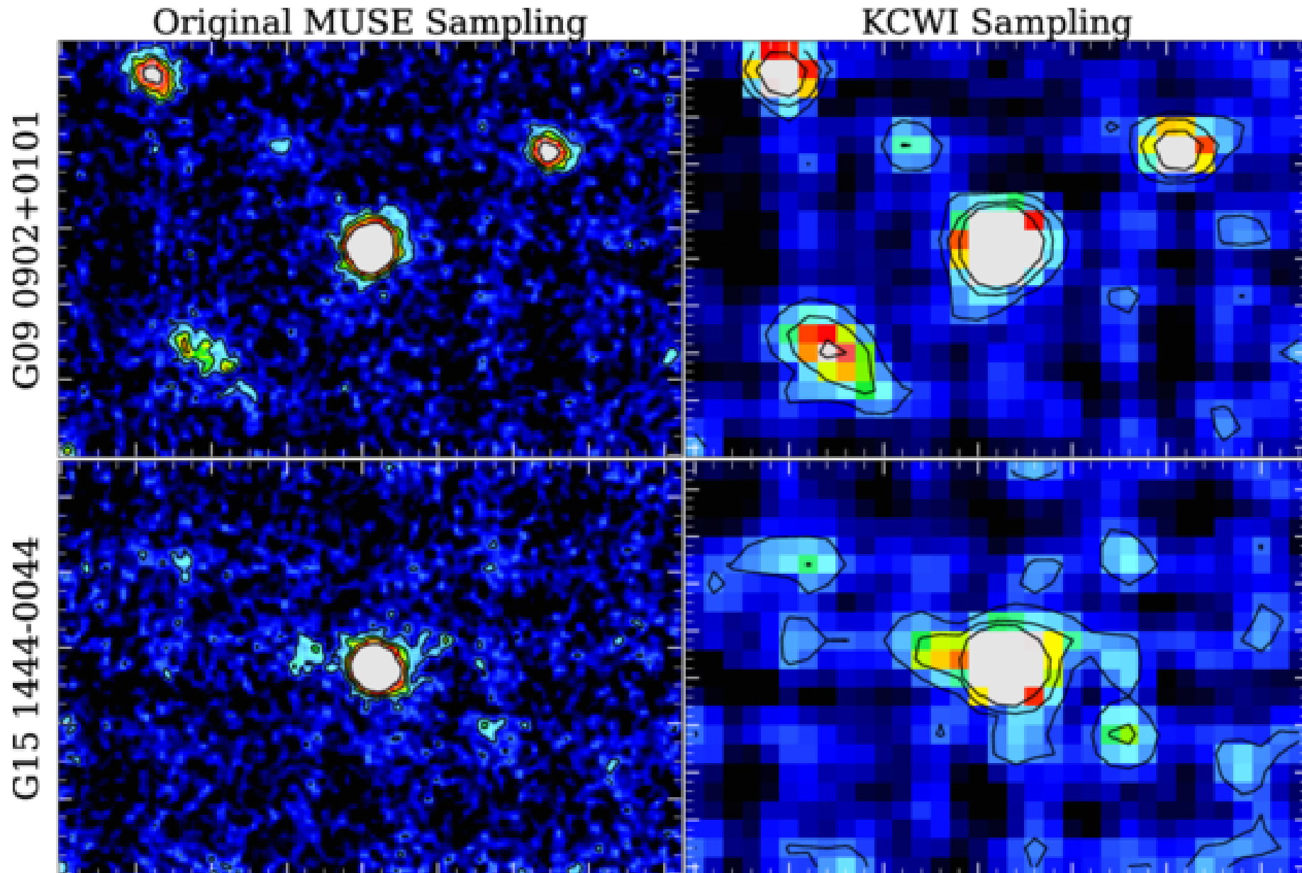
Figure 2. from Kevin Hall and Hai Fu 2026 Astrophys. J. 1002 doi:10.3847/1538-4357/ae6065 https://dx.doi.org/10.3847/1538-4357/ae6065 © 2026. The Author(s). Published by the American Astronomical Society.
