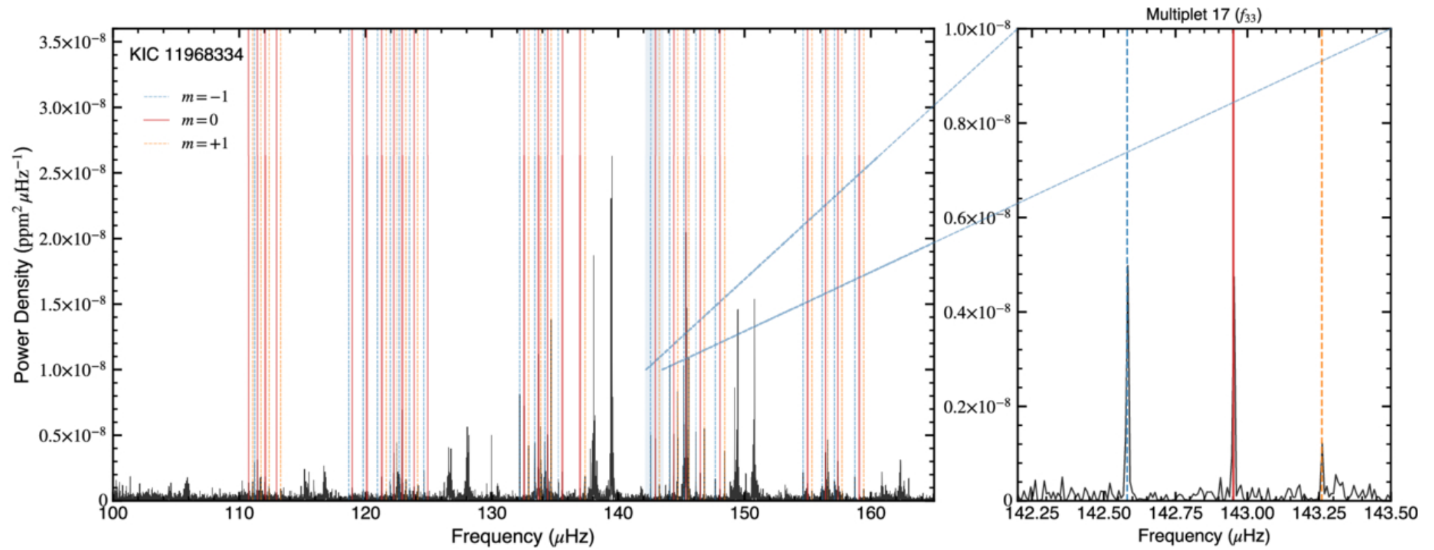
Figure 9. from Xinyi Zhang et al 2026 Astrophys. J. 1002 doi:10.3847/1538-4357/ae5e61 https://dx.doi.org/10.3847/1538-4357/ae5e61 © 2026. The Author(s). Published by the American Astronomical Society.
