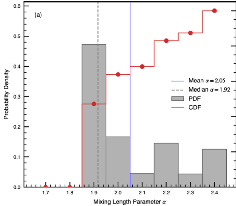
Figure 8. from Xinyi Zhang et al 2026 Astrophys. J. 1002 doi:10.3847/1538-4357/ae5e61 https://dx.doi.org/10.3847/1538-4357/ae5e61 © 2026. The Author(s). Published by the American Astronomical Society.
