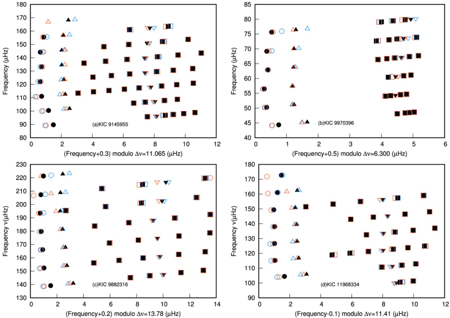
Figure 6. from Xinyi Zhang et al 2026 Astrophys. J. 1002 doi:10.3847/1538-4357/ae5e61 https://dx.doi.org/10.3847/1538-4357/ae5e61 © 2026. The Author(s). Published by the American Astronomical Society.
