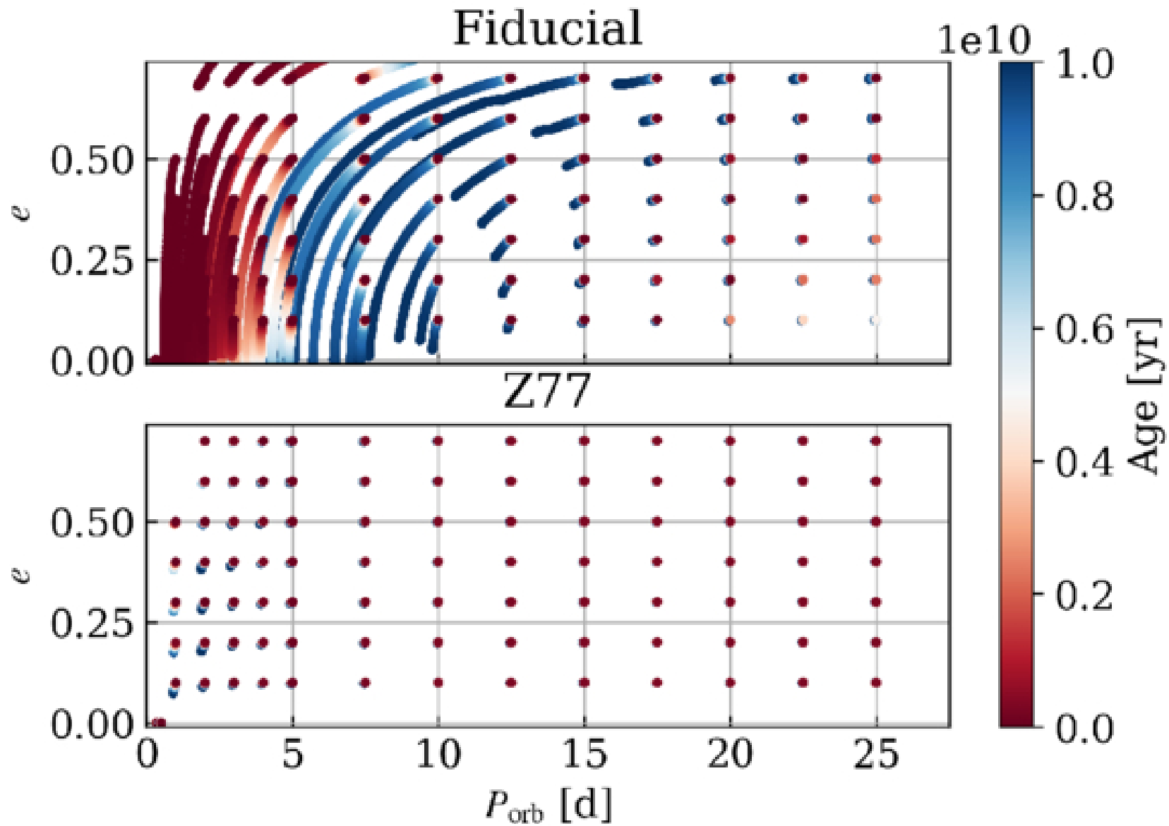
Figure 4. from Veome Kapil et al 2026 Astrophys. J. 1002 doi:10.3847/1538-4357/ae5e48 https://dx.doi.org/10.3847/1538-4357/ae5e48 © 2026. The Author(s). Published by the American Astronomical Society.
