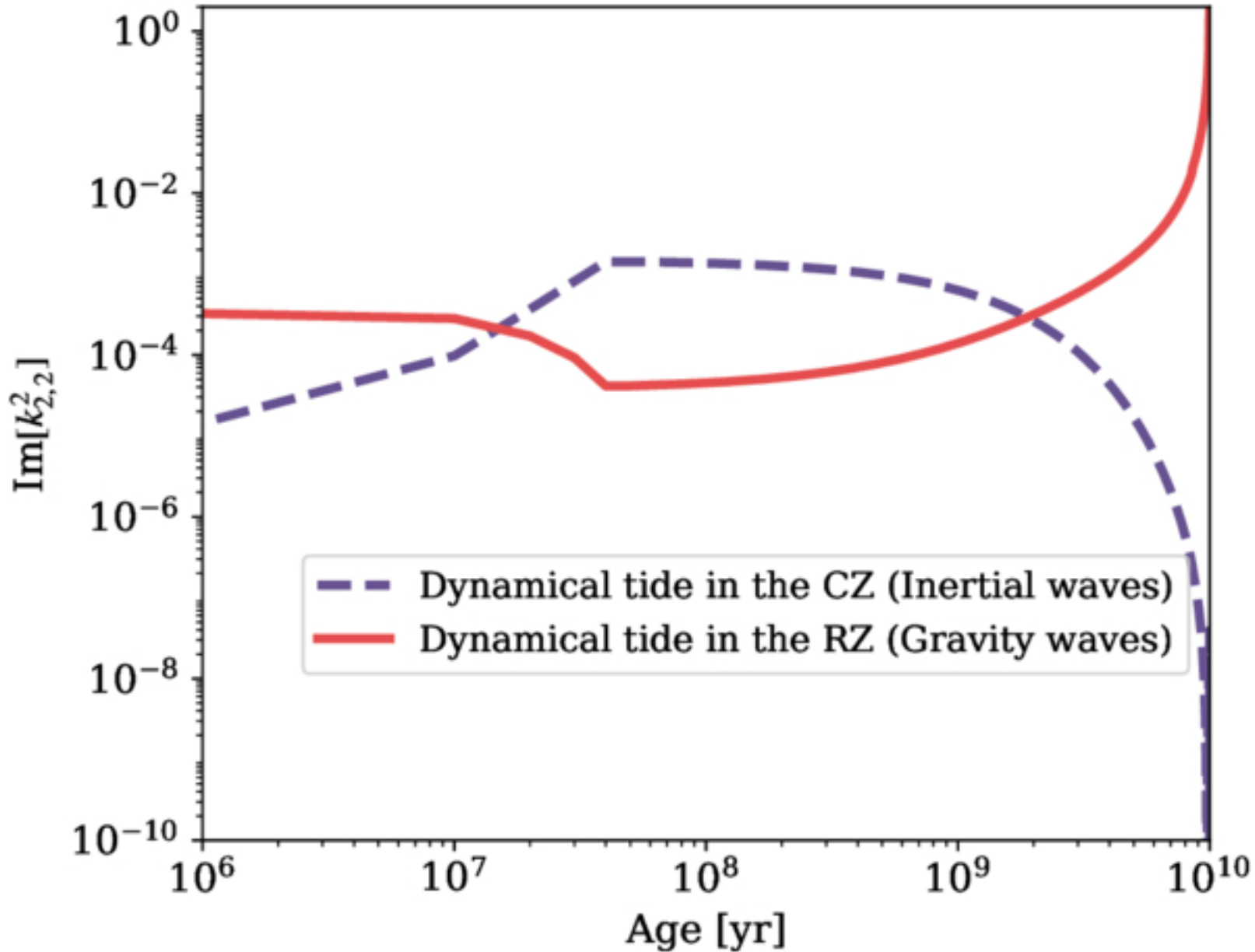
Figure 11. from Veome Kapil et al 2026 Astrophys. J. 1002 doi:10.3847/1538-4357/ae5e48 https://dx.doi.org/10.3847/1538-4357/ae5e48 © 2026. The Author(s). Published by the American Astronomical Society.
