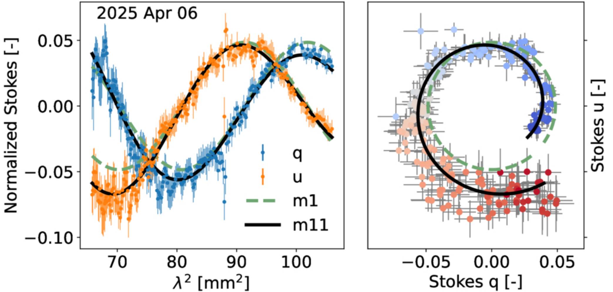
Figure 3. from Joseph M. Michail et al 2026 Astrophys. J. 1003 doi:10.3847/1538-4357/ae5dc8 https://dx.doi.org/10.3847/1538-4357/ae5dc8 © 2026. The Author(s). Published by the American Astronomical Society.
