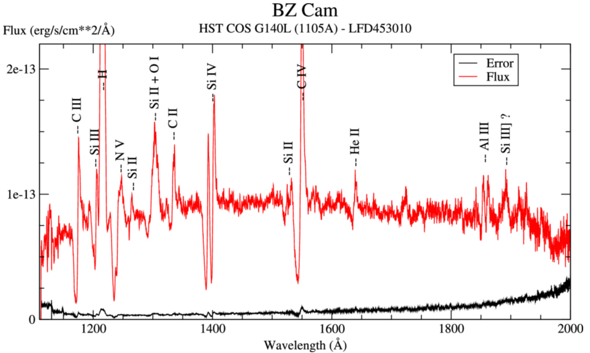
Figure 6. from ölen Balman et al 2026 Astrophys. J. 1003 doi:10.3847/1538-4357/ae5db6 https://dx.doi.org/10.3847/1538-4357/ae5db6 © 2026. The Author(s). Published by the American Astronomical Society.
