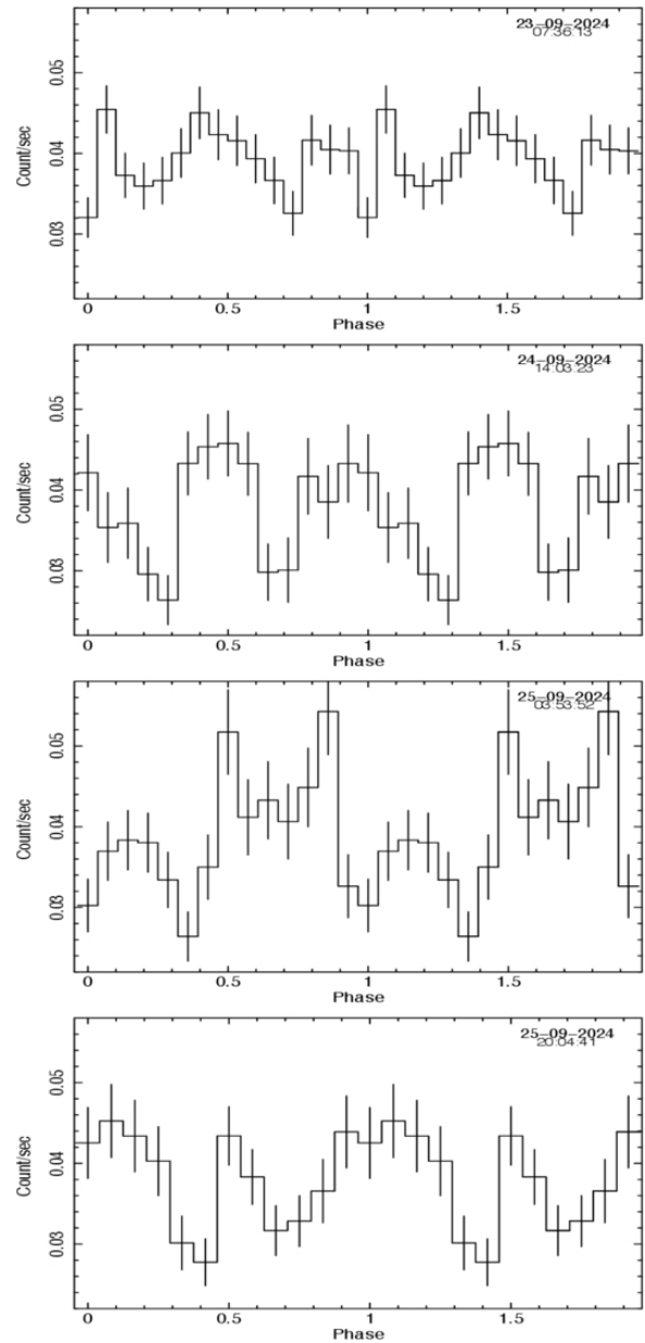
Figure 4. from ölen Balman et al 2026 Astrophys. J. 1003 doi:10.3847/1538-4357/ae5db6 https://dx.doi.org/10.3847/1538-4357/ae5db6 © 2026. The Author(s). Published by the American Astronomical Society.
