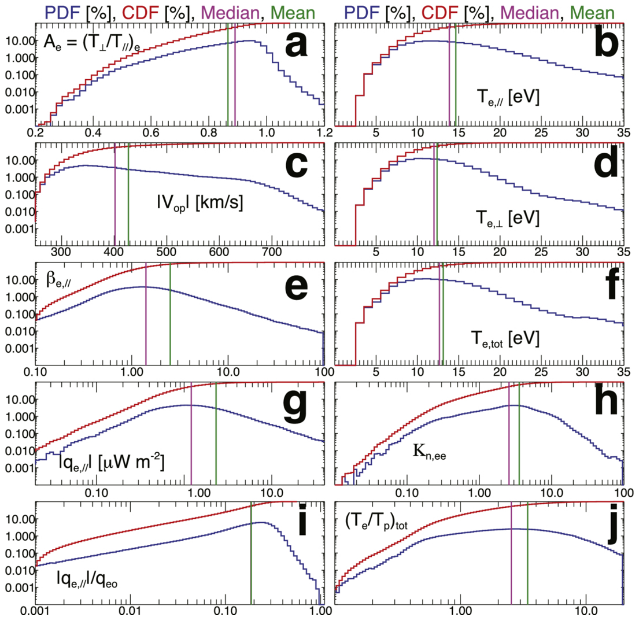
Figure 6. from Lynn B. Wilson et al 2026 Astrophys. J. 1002 doi:10.3847/1538-4357/ae5d4a https://dx.doi.org/10.3847/1538-4357/ae5d4a © 2026. The Author(s). Published by the American Astronomical Society.
