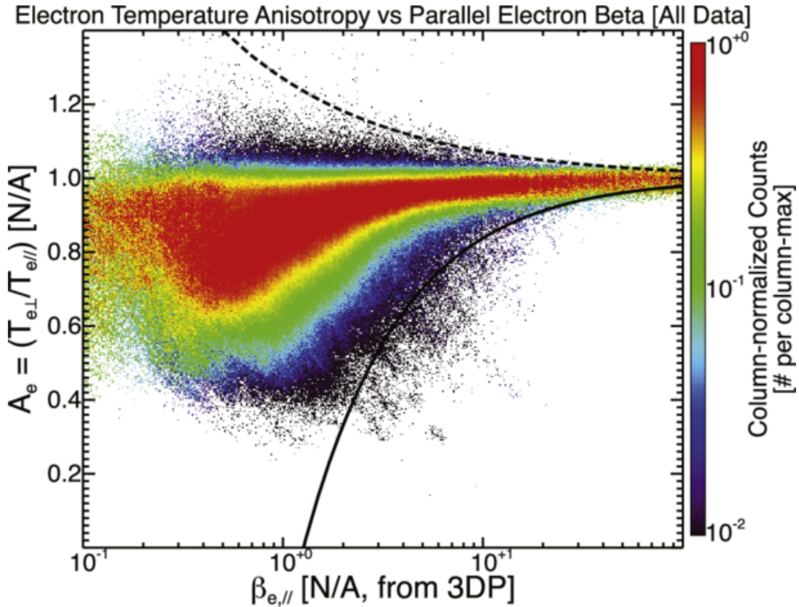
Figure 5. from Lynn B. Wilson et al 2026 Astrophys. J. 1002 doi:10.3847/1538-4357/ae5d4a https://dx.doi.org/10.3847/1538-4357/ae5d4a © 2026. The Author(s). Published by the American Astronomical Society.
