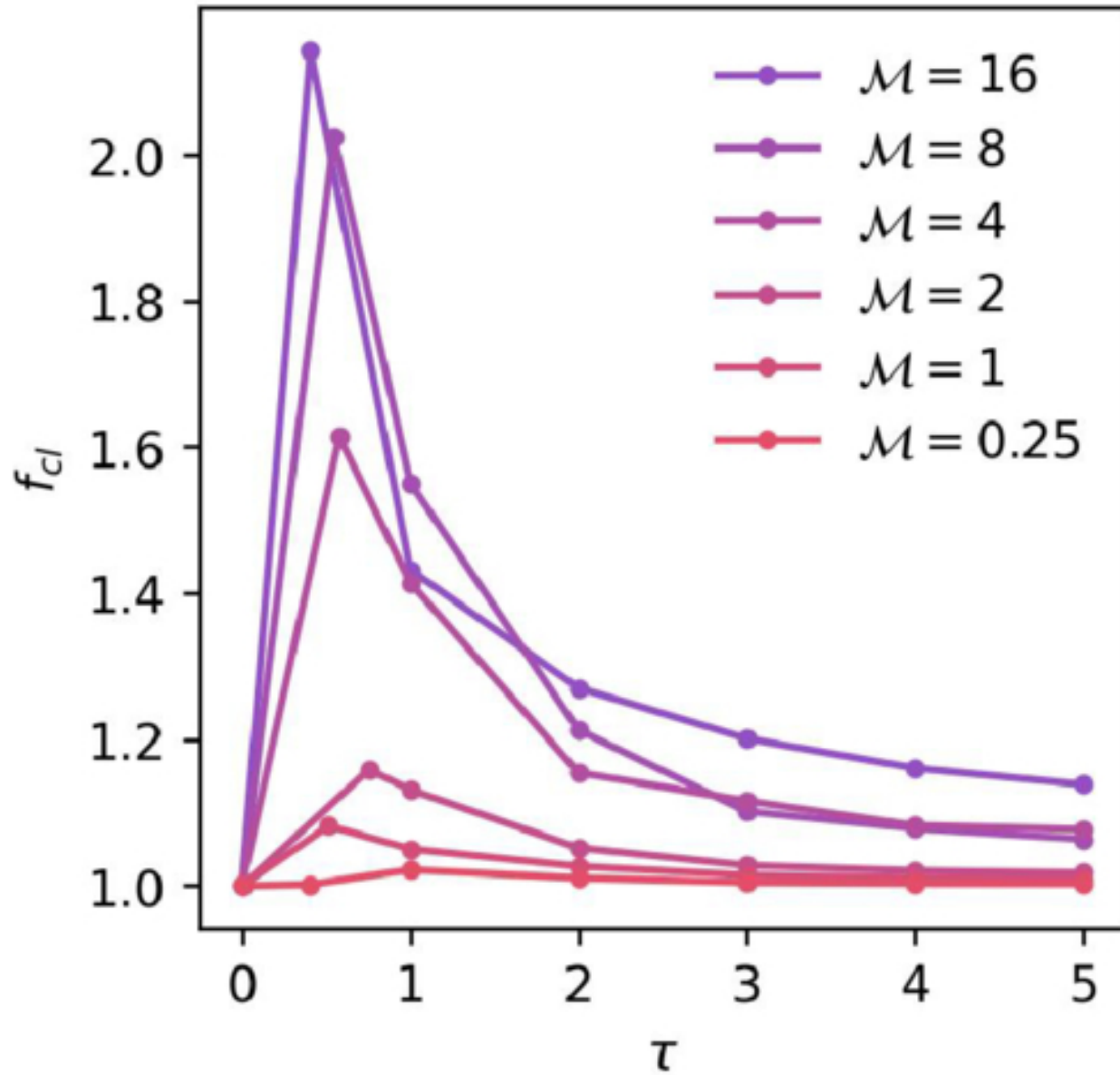
Figure 6. from Keyan Gootkin et al 2026 Astrophys. J. 1003 doi:10.3847/1538-4357/ae5d42 https://dx.doi.org/10.3847/1538-4357/ae5d42 © 2026. The Author(s). Published by the American Astronomical Society.
