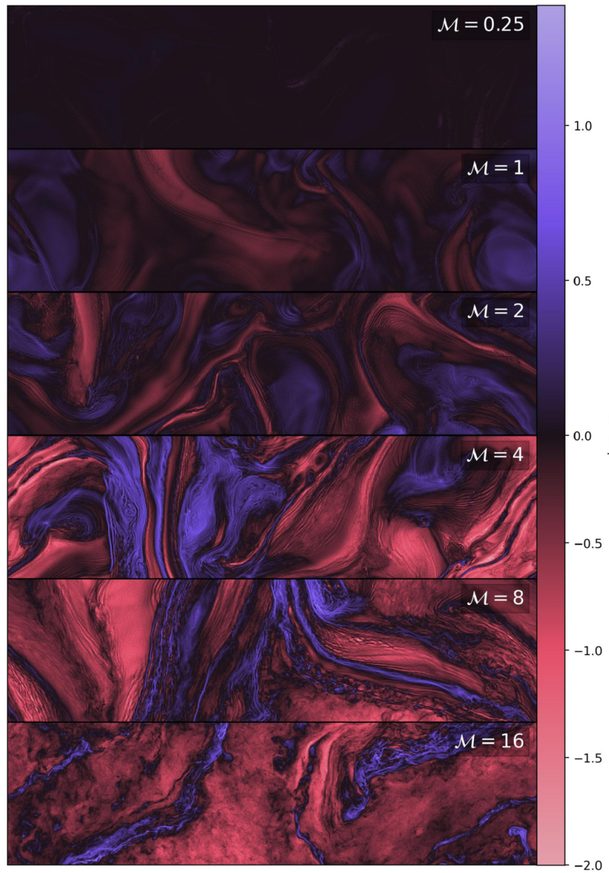
Figure 5. from Keyan Gootkin et al 2026 Astrophys. J. 1003 doi:10.3847/1538-4357/ae5d42 https://dx.doi.org/10.3847/1538-4357/ae5d42 © 2026. The Author(s). Published by the American Astronomical Society.
