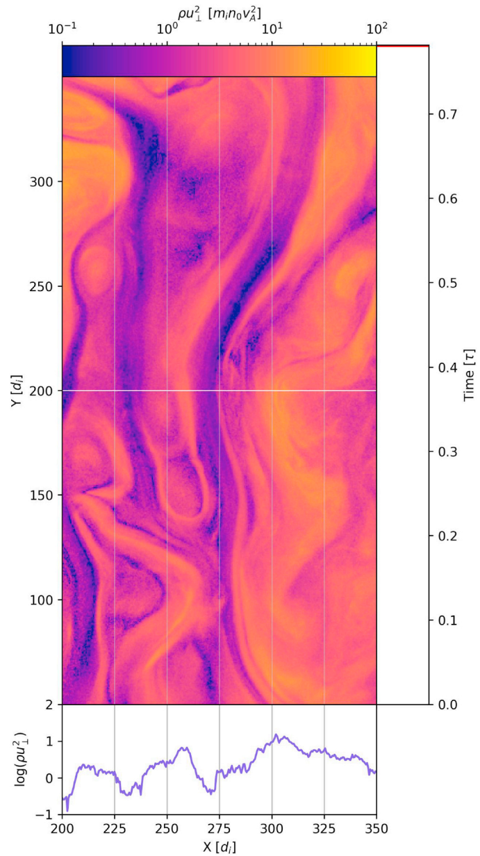
Figure 18. from Keyan Gootkin et al 2026 Astrophys. J. 1003 doi:10.3847/1538-4357/ae5d42 https://dx.doi.org/10.3847/1538-4357/ae5d42 © 2026. The Author(s). Published by the American Astronomical Society.
