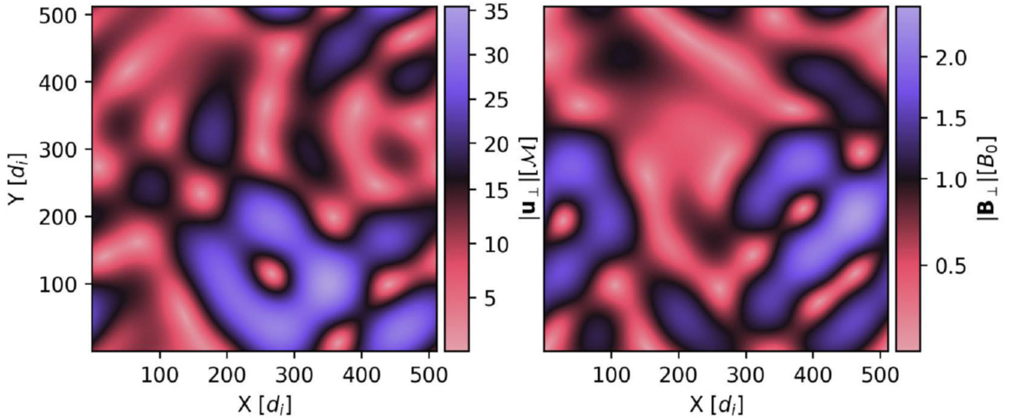
Figure 1. from Keyan Gootkin et al 2026 Astrophys. J. 1003 doi:10.3847/1538-4357/ae5d42 https://dx.doi.org/10.3847/1538-4357/ae5d42 © 2026. The Author(s). Published by the American Astronomical Society.
