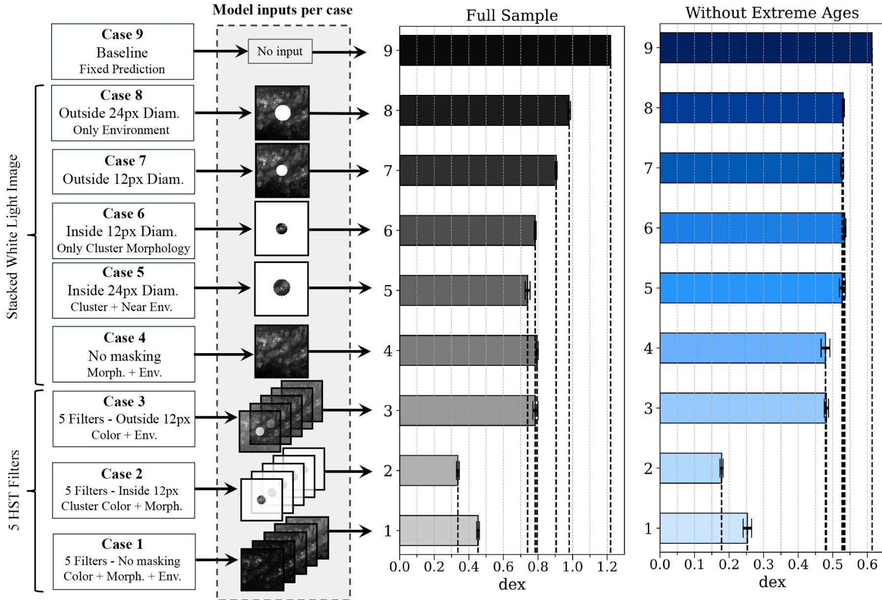
Figure 5. from Javier Viaña et al 2026 Astrophys. J. 1004 doi:10.3847/1538-4357/ae5d31 https://dx.doi.org/10.3847/1538-4357/ae5d31 © 2026. The Author(s). Published by the American Astronomical Society.
