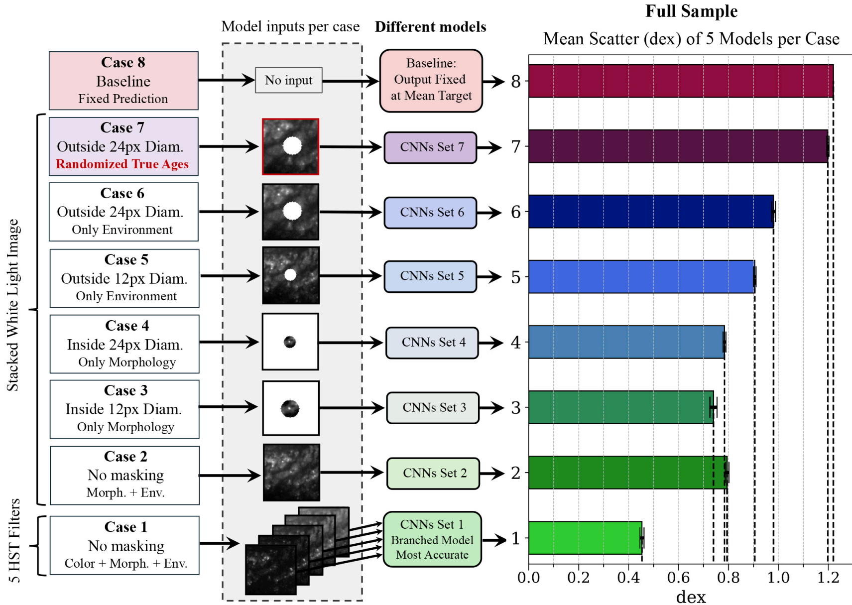
Figure 4. from Javier Viaña et al 2026 Astrophys. J. 1004 doi:10.3847/1538-4357/ae5d31 https://dx.doi.org/10.3847/1538-4357/ae5d31 © 2026. The Author(s). Published by the American Astronomical Society.
