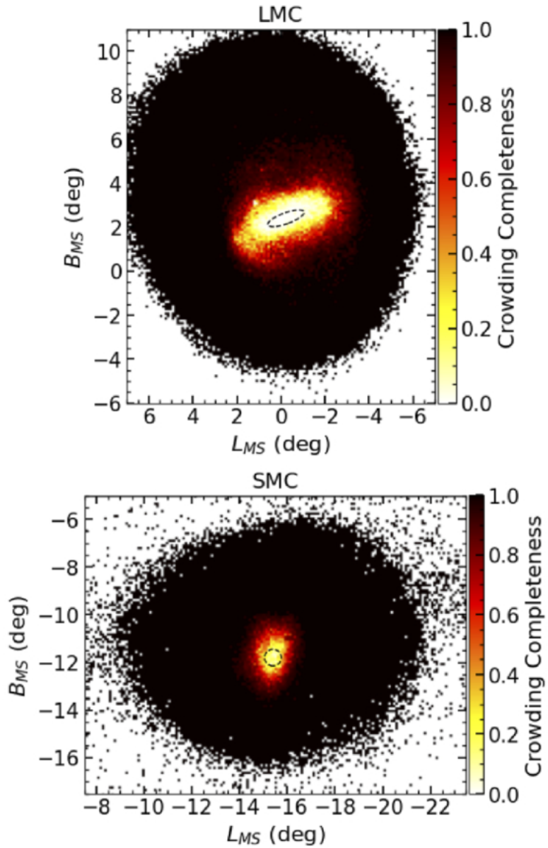
Figure 5. from Slater J. Oden et al 2026 Astrophys. J. 1003 doi:10.3847/1538-4357/ae5c9e https://dx.doi.org/10.3847/1538-4357/ae5c9e © 2026. The Author(s). Published by the American Astronomical Society.
