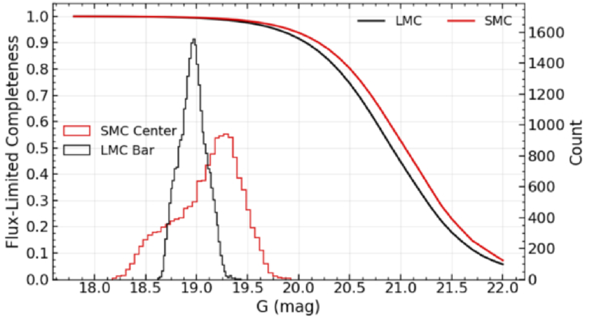
Figure 4. from Slater J. Oden et al 2026 Astrophys. J. 1003 doi:10.3847/1538-4357/ae5c9e https://dx.doi.org/10.3847/1538-4357/ae5c9e © 2026. The Author(s). Published by the American Astronomical Society.
