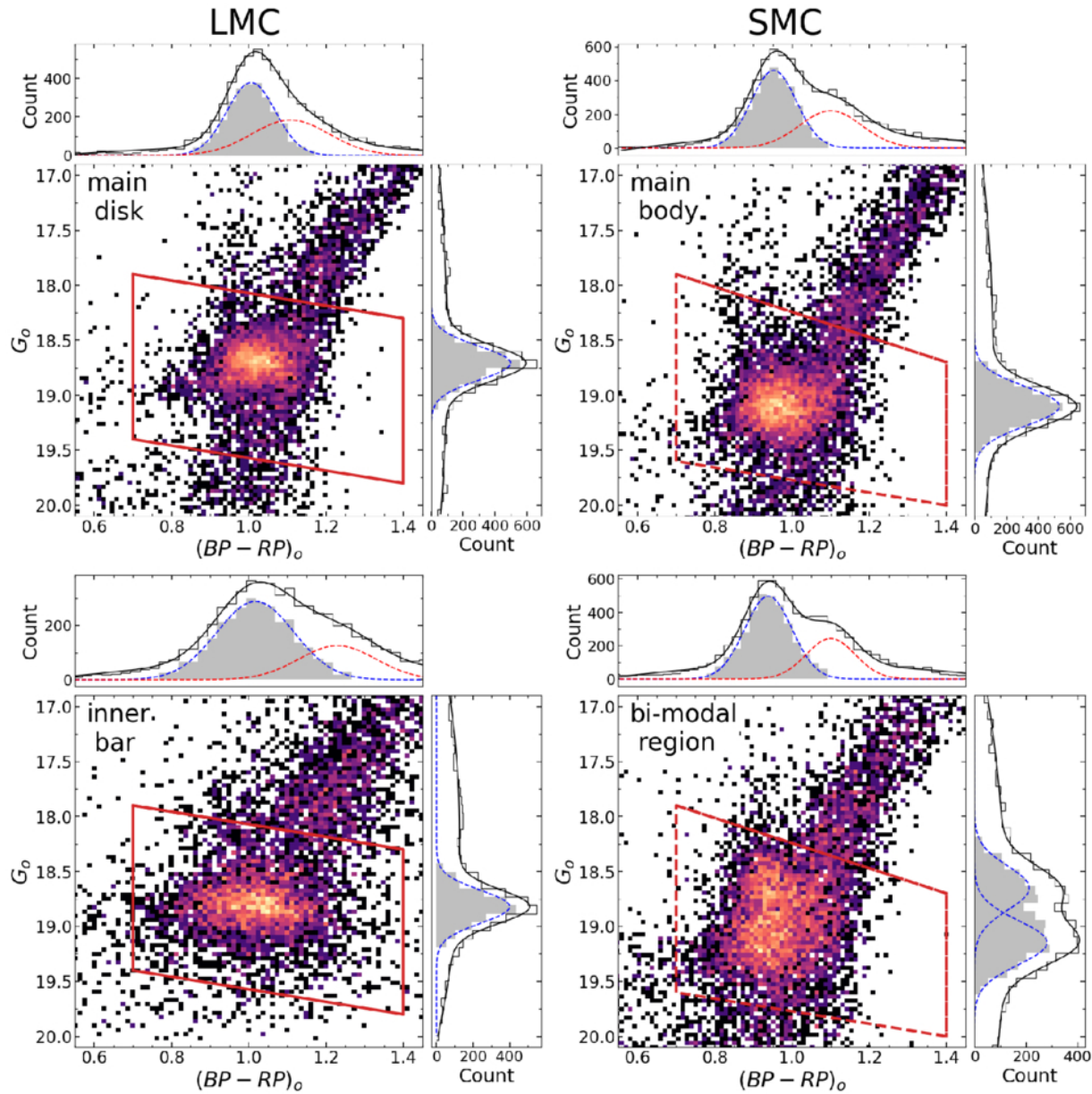
Figure 3. from Slater J. Oden et al 2026 Astrophys. J. 1003 doi:10.3847/1538-4357/ae5c9e https://dx.doi.org/10.3847/1538-4357/ae5c9e © 2026. The Author(s). Published by the American Astronomical Society.
