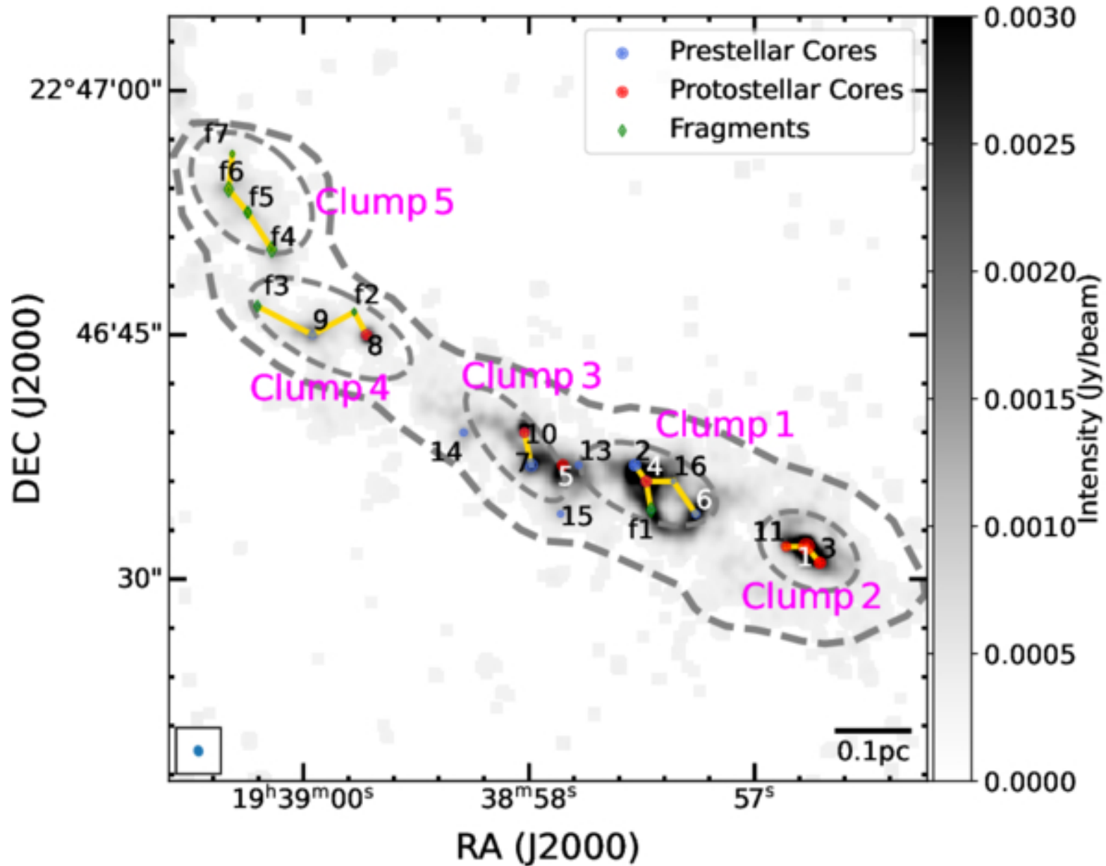
Figure 3. from Chengzhi Meng et al 2026 Astrophys. J. 1002 doi:10.3847/1538-4357/ae5b7f https://dx.doi.org/10.3847/1538-4357/ae5b7f © 2026. The Author(s). Published by the American Astronomical Society.
