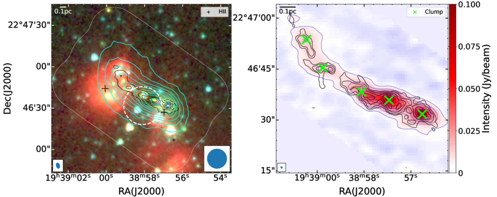
Figure 1. from Chengzhi Meng et al 2026 Astrophys. J. 1002 doi:10.3847/1538-4357/ae5b7f https://dx.doi.org/10.3847/1538-4357/ae5b7f © 2026. The Author(s). Published by the American Astronomical Society.
