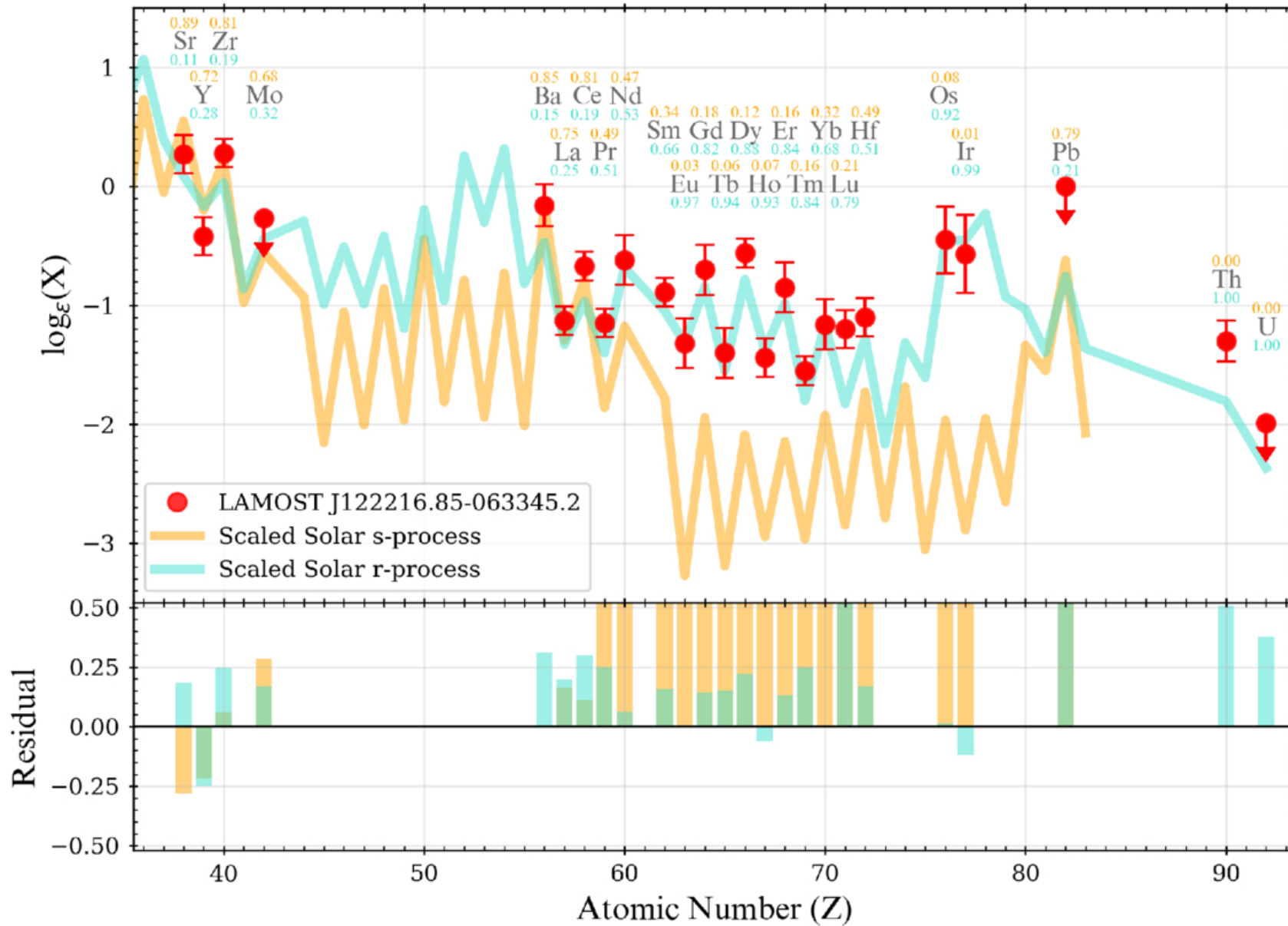
Figure 5. from Miji Jeong et al 2026 Astrophys. J. 1005 doi:10.3847/1538-4357/ae5b7d https://dx.doi.org/10.3847/1538-4357/ae5b7d © 2026. The Author(s). Published by the American Astronomical Society.
