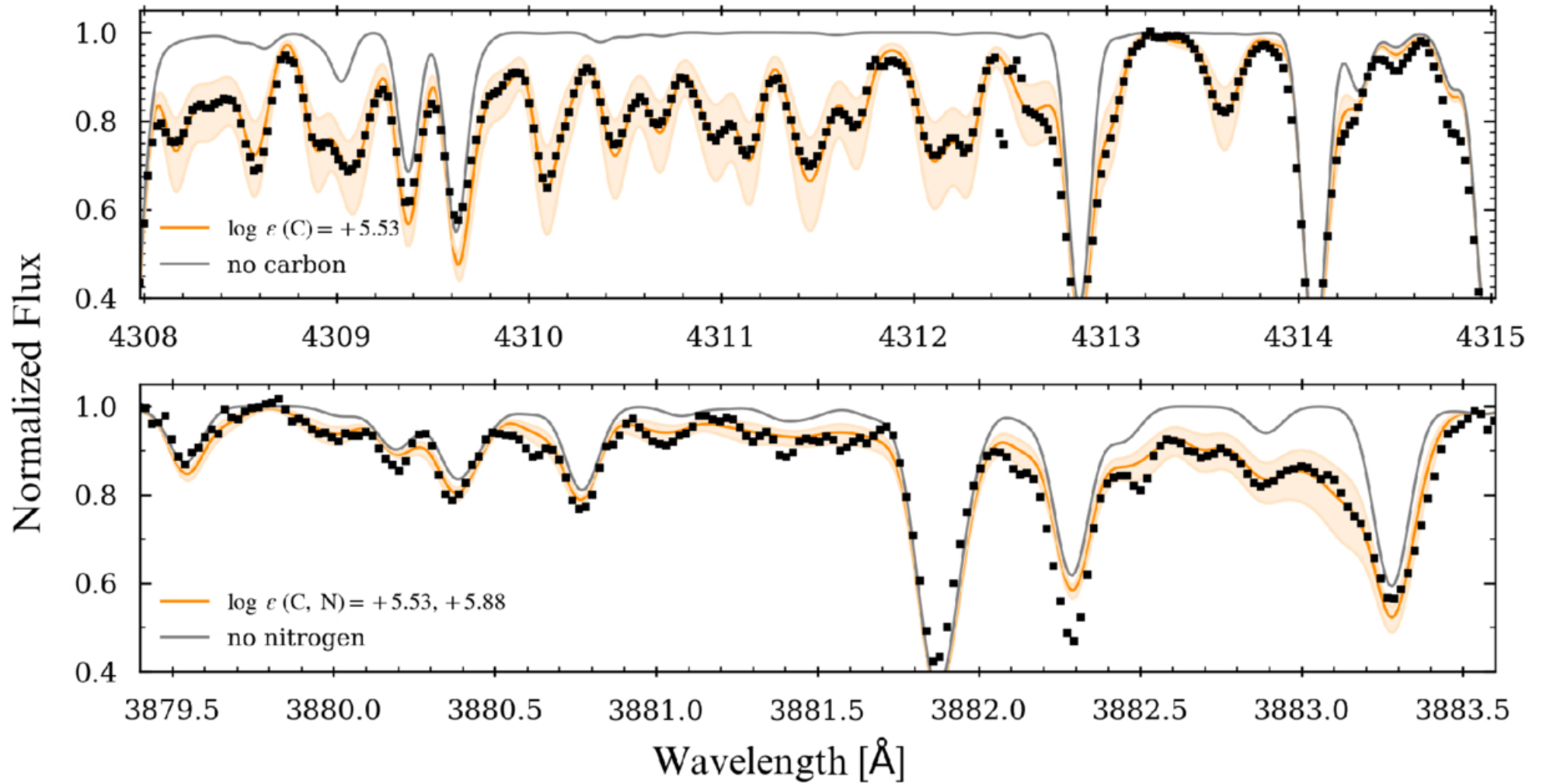
Figure 3. from Miji Jeong et al 2026 Astrophys. J. 1005 doi:10.3847/1538-4357/ae5b7d https://dx.doi.org/10.3847/1538-4357/ae5b7d © 2026. The Author(s). Published by the American Astronomical Society.
