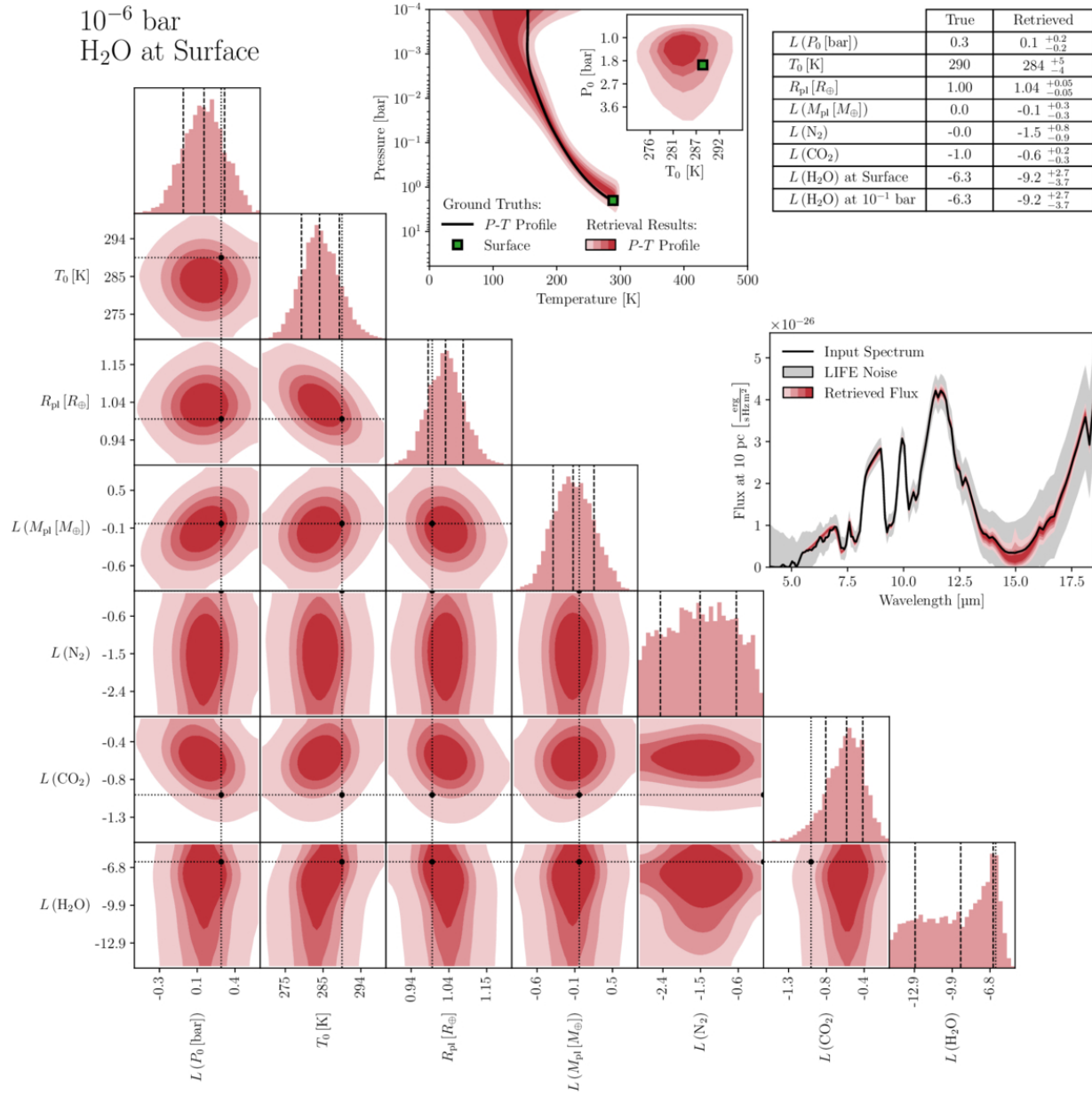
Figure 8. from S. Rugheimer et al 2026 Astrophys. J. 1003 doi:10.3847/1538-4357/ae5b75 https://dx.doi.org/10.3847/1538-4357/ae5b75 © 2026. The Author(s). Published by the American Astronomical Society.
