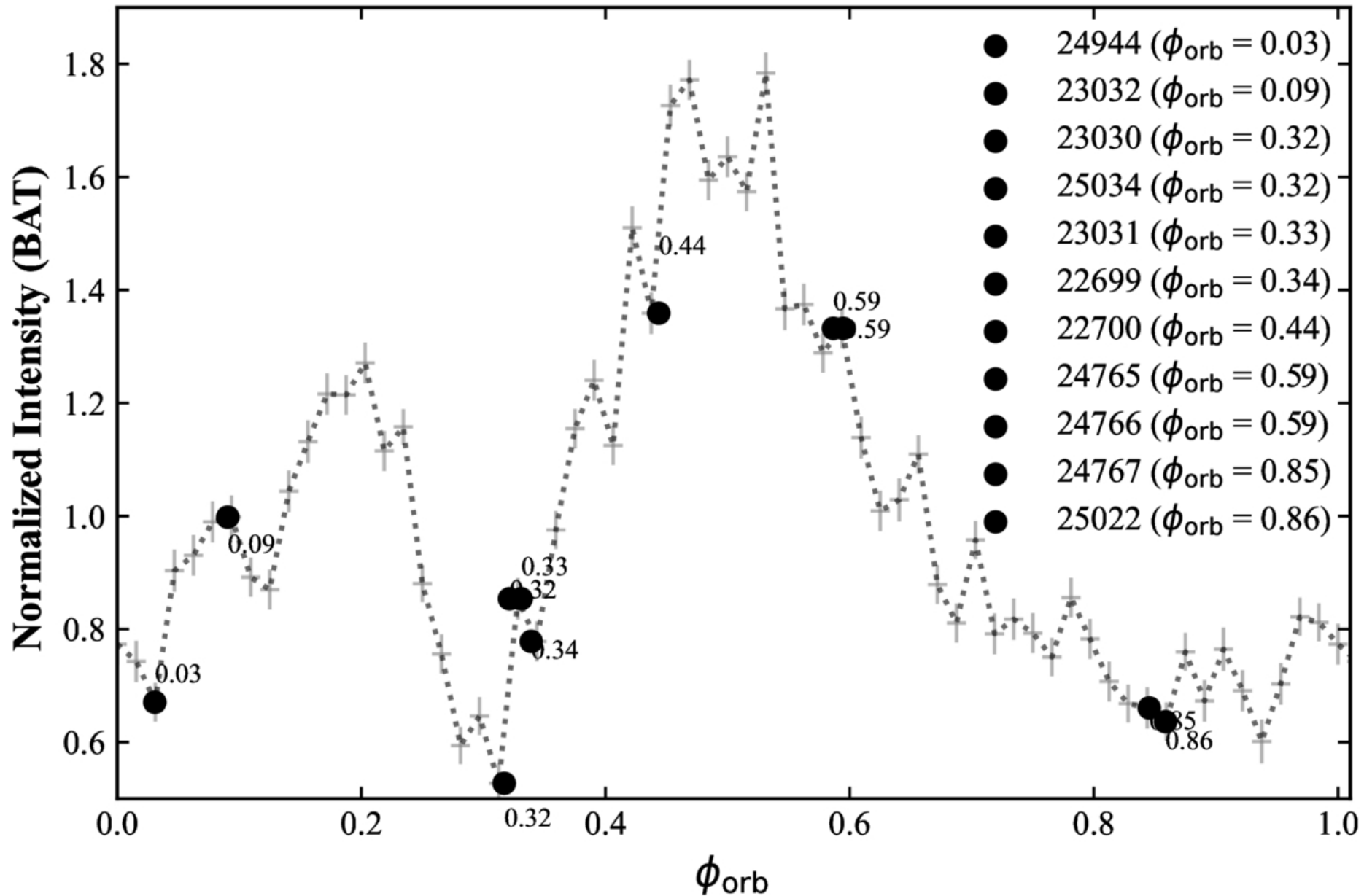
Figure 1. from Pragati Pradhan et al 2026 Astrophys. J. 1004 doi:10.3847/1538-4357/ae5b71 https://dx.doi.org/10.3847/1538-4357/ae5b71 © 2026. The Author(s). Published by the American Astronomical Society.
