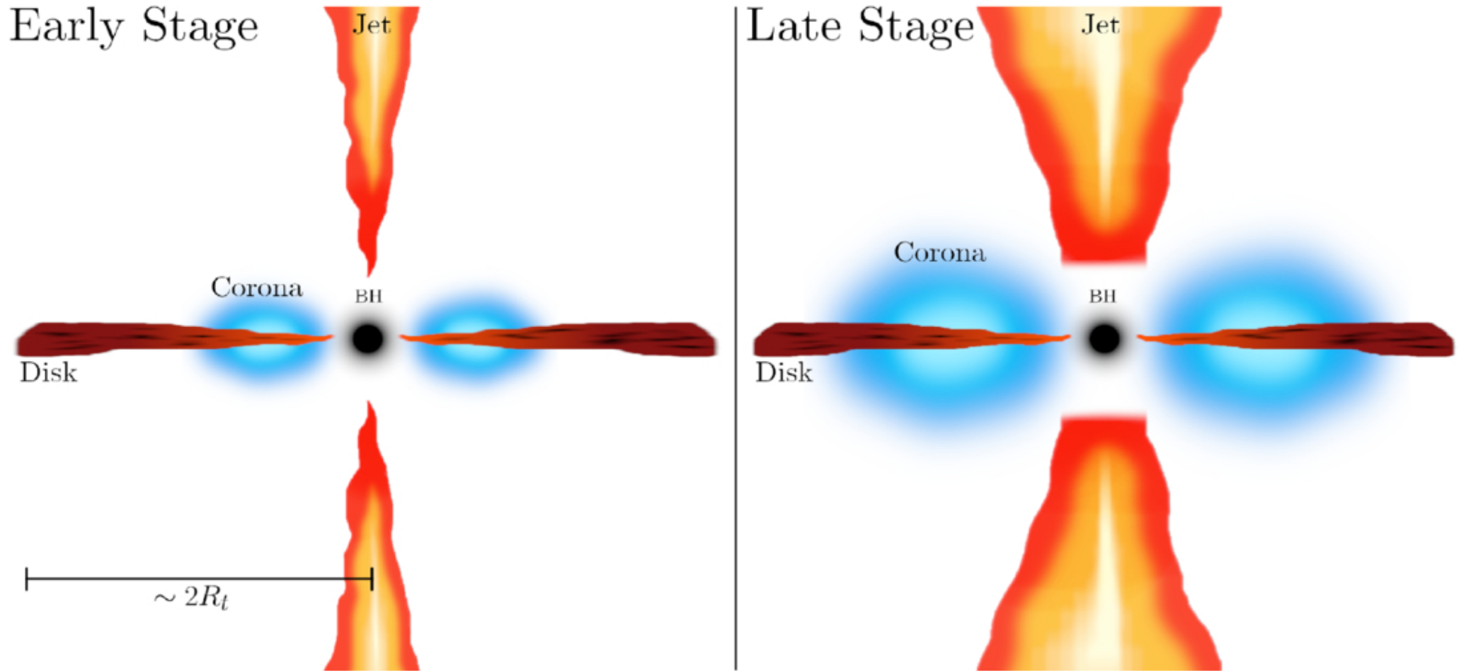
Figure 9. from Arka Chatterjee et al 2026 Astrophys. J. 1002 doi:10.3847/1538-4357/ae5b6f https://dx.doi.org/10.3847/1538-4357/ae5b6f © 2026. The Author(s). Published by the American Astronomical Society.
