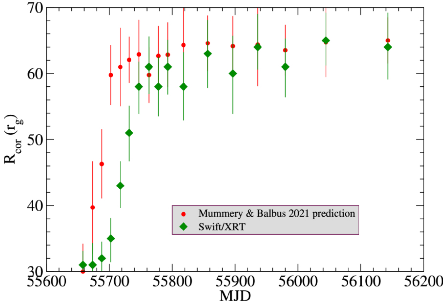
Figure 8. from Arka Chatterjee et al 2026 Astrophys. J. 1002 doi:10.3847/1538-4357/ae5b6f https://dx.doi.org/10.3847/1538-4357/ae5b6f © 2026. The Author(s). Published by the American Astronomical Society.
