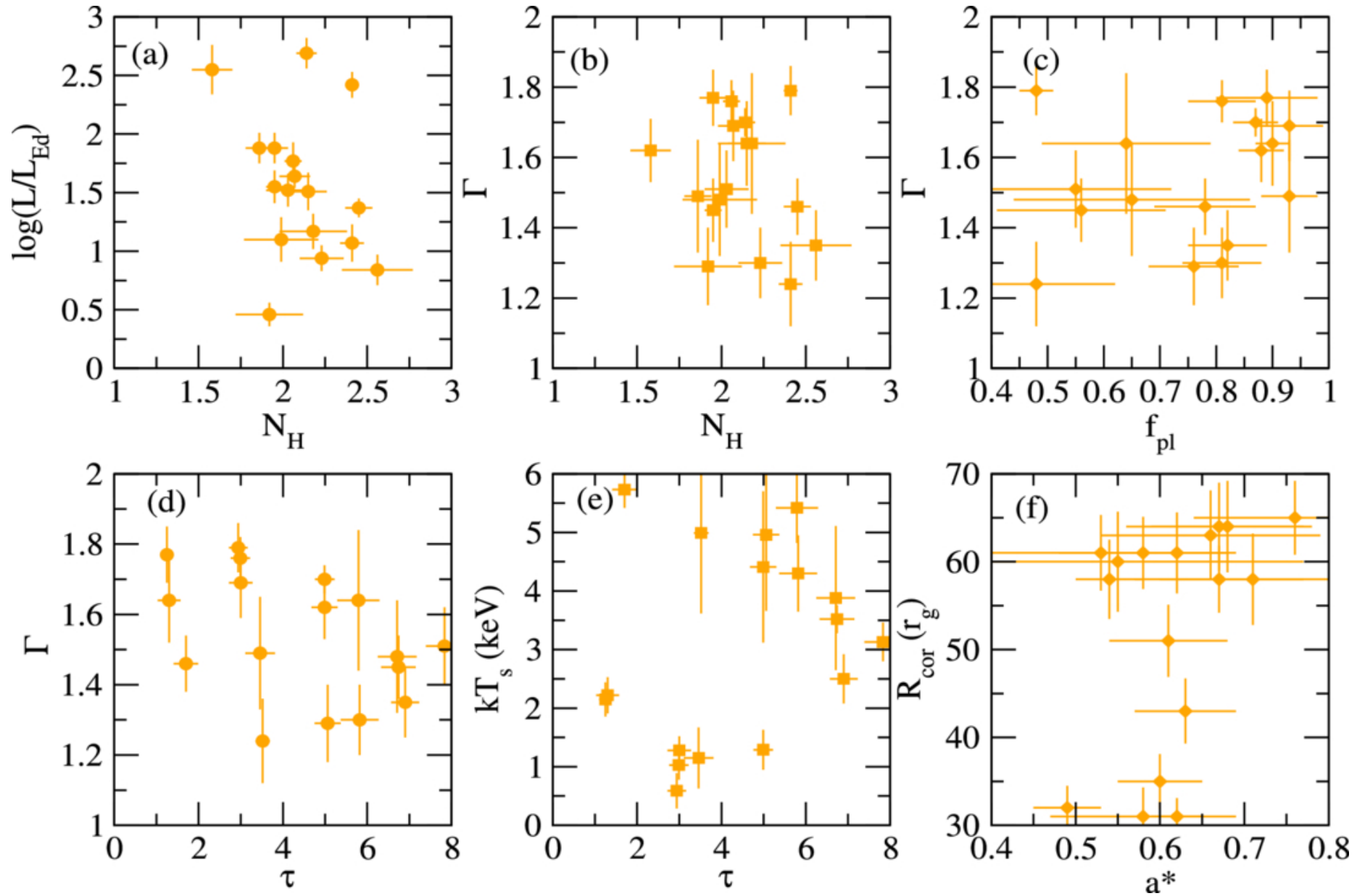
Figure 6. from Arka Chatterjee et al 2026 Astrophys. J. 1002 doi:10.3847/1538-4357/ae5b6f https://dx.doi.org/10.3847/1538-4357/ae5b6f © 2026. The Author(s). Published by the American Astronomical Society.
