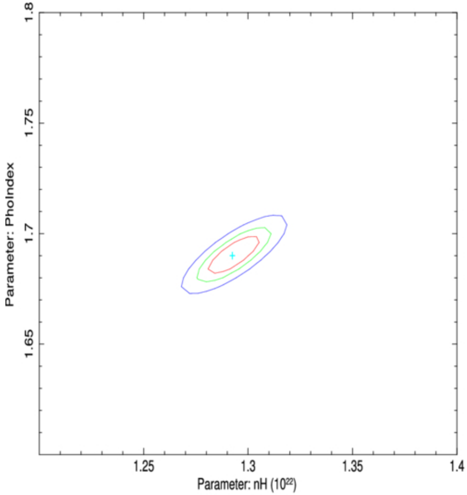
Figure 4. from Arka Chatterjee et al 2026 Astrophys. J. 1002 doi:10.3847/1538-4357/ae5b6f https://dx.doi.org/10.3847/1538-4357/ae5b6f © 2026. The Author(s). Published by the American Astronomical Society.
