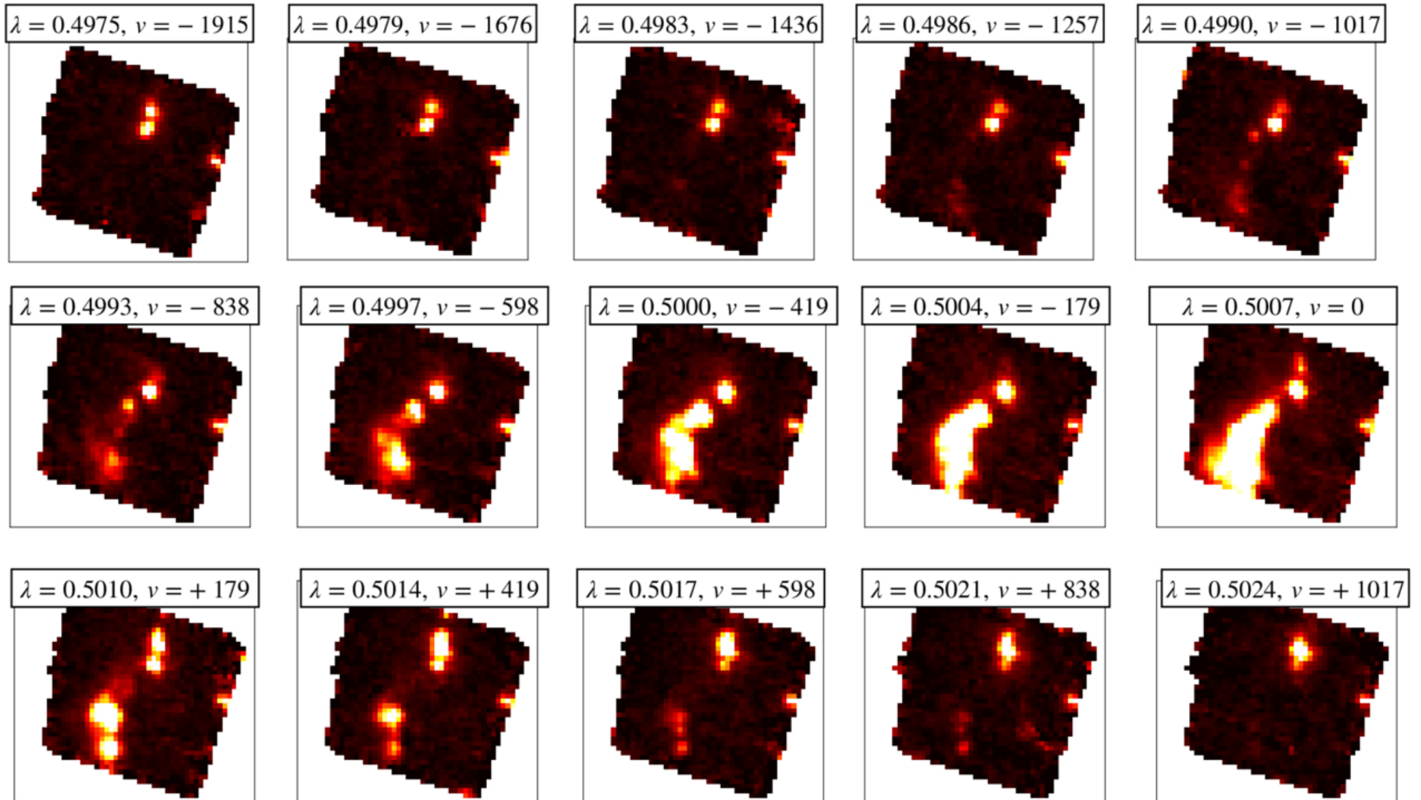
Figure 7. from Namrata Roy et al 2026 Astrophys. J. 1002 doi:10.3847/1538-4357/ae5b68 https://dx.doi.org/10.3847/1538-4357/ae5b68 © 2026. The Author(s). Published by the American Astronomical Society.
