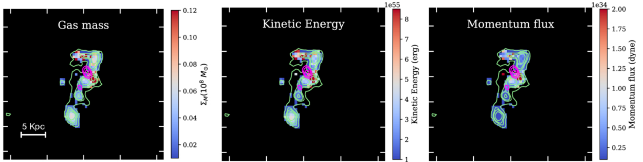
Figure 6. from Namrata Roy et al 2026 Astrophys. J. 1002 doi:10.3847/1538-4357/ae5b68 https://dx.doi.org/10.3847/1538-4357/ae5b68 © 2026. The Author(s). Published by the American Astronomical Society.
