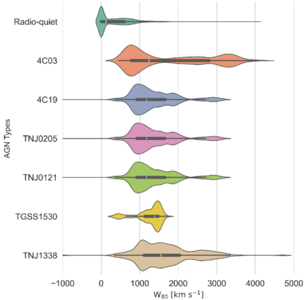
Figure 20. from Namrata Roy et al 2026 Astrophys. J. 1002 doi:10.3847/1538-4357/ae5b68 https://dx.doi.org/10.3847/1538-4357/ae5b68 © 2026. The Author(s). Published by the American Astronomical Society.
