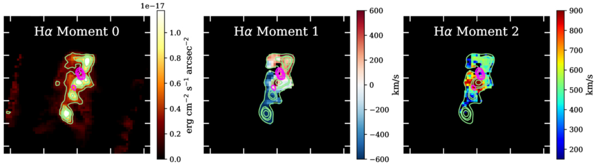
Figure 2. from Namrata Roy et al 2026 Astrophys. J. 1002 doi:10.3847/1538-4357/ae5b68 https://dx.doi.org/10.3847/1538-4357/ae5b68 © 2026. The Author(s). Published by the American Astronomical Society.
