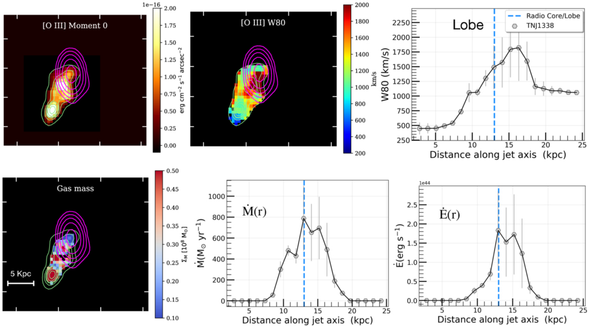
Figure 19. from Namrata Roy et al 2026 Astrophys. J. 1002 doi:10.3847/1538-4357/ae5b68 https://dx.doi.org/10.3847/1538-4357/ae5b68 © 2026. The Author(s). Published by the American Astronomical Society.
