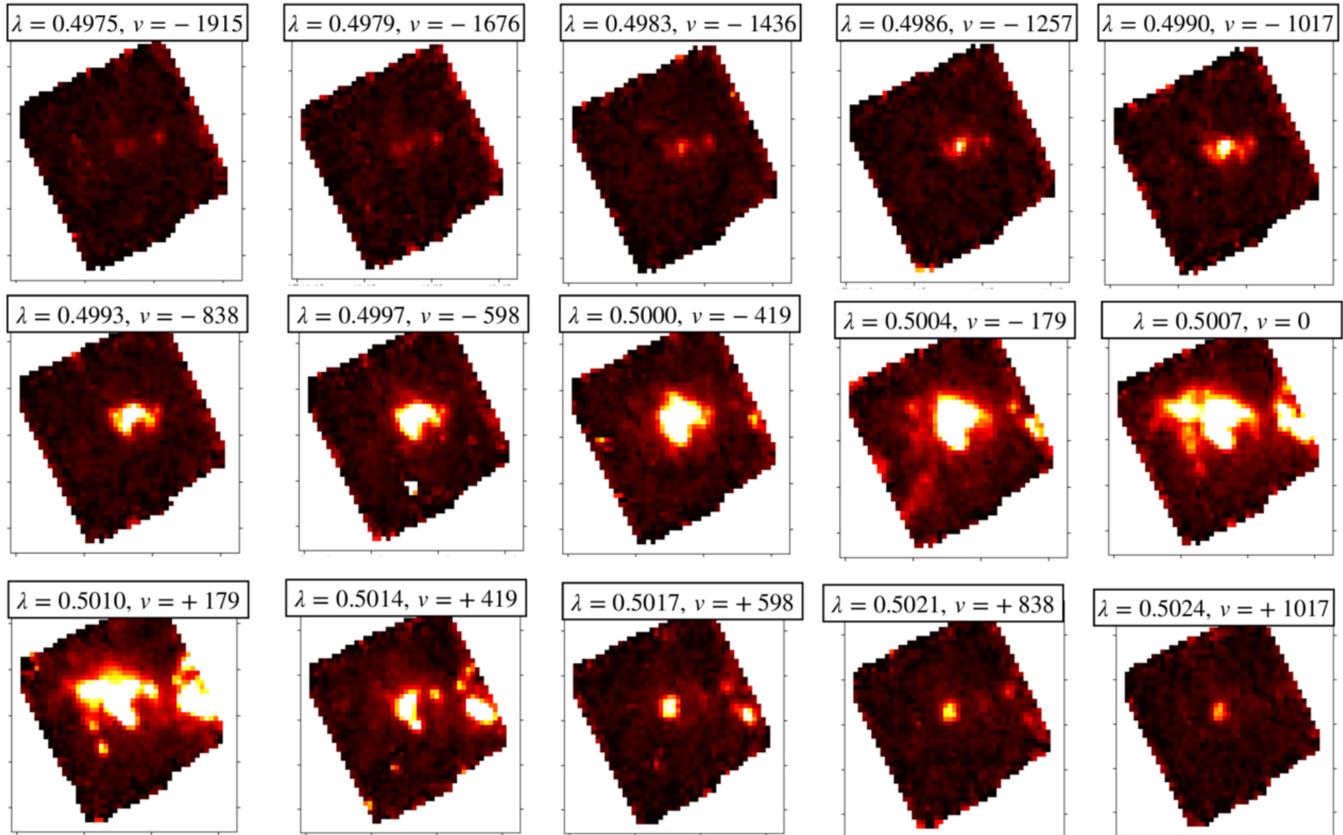
Figure 16. from Namrata Roy et al 2026 Astrophys. J. 1002 doi:10.3847/1538-4357/ae5b68 https://dx.doi.org/10.3847/1538-4357/ae5b68 © 2026. The Author(s). Published by the American Astronomical Society.
