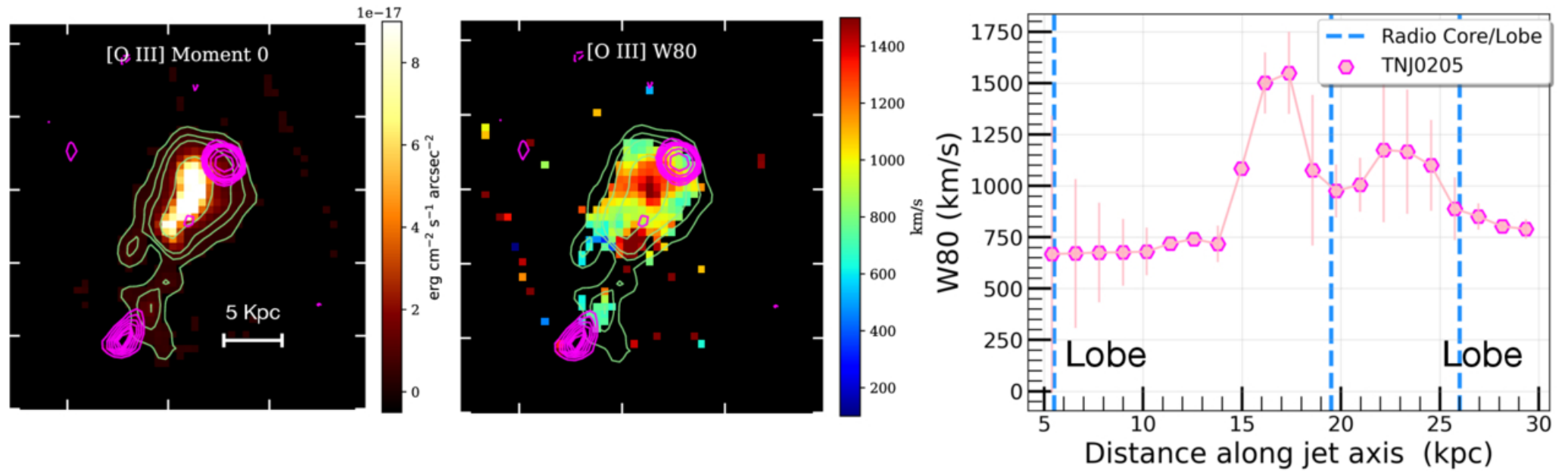
Figure 14. from Namrata Roy et al 2026 Astrophys. J. 1002 doi:10.3847/1538-4357/ae5b68 https://dx.doi.org/10.3847/1538-4357/ae5b68 © 2026. The Author(s). Published by the American Astronomical Society.
