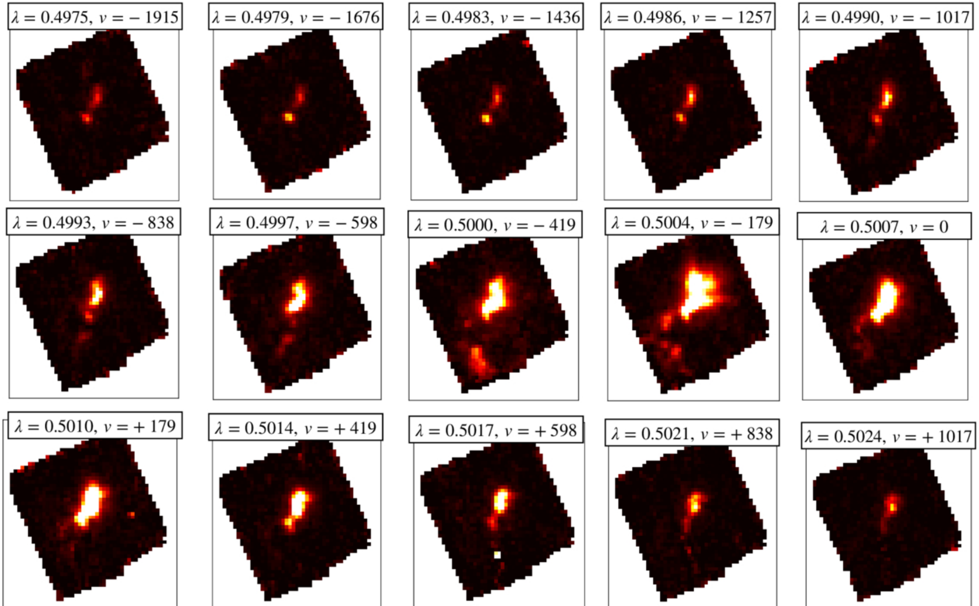
Figure 13. from Namrata Roy et al 2026 Astrophys. J. 1002 doi:10.3847/1538-4357/ae5b68 https://dx.doi.org/10.3847/1538-4357/ae5b68 © 2026. The Author(s). Published by the American Astronomical Society.
